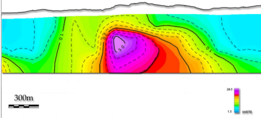
Figure 2: IP Chargeability anomaly
