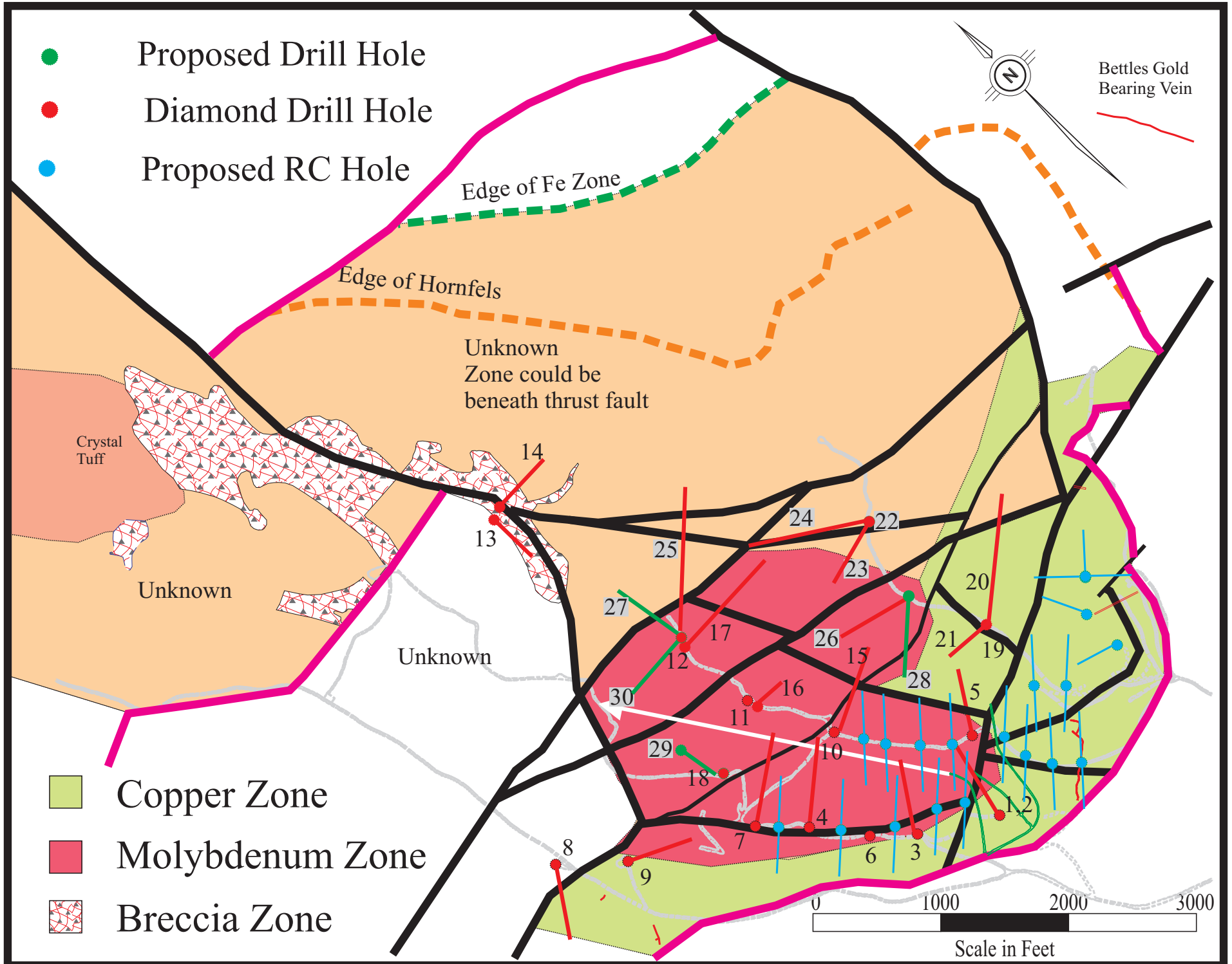
Figure 1: Pine Tree Drill Plan
