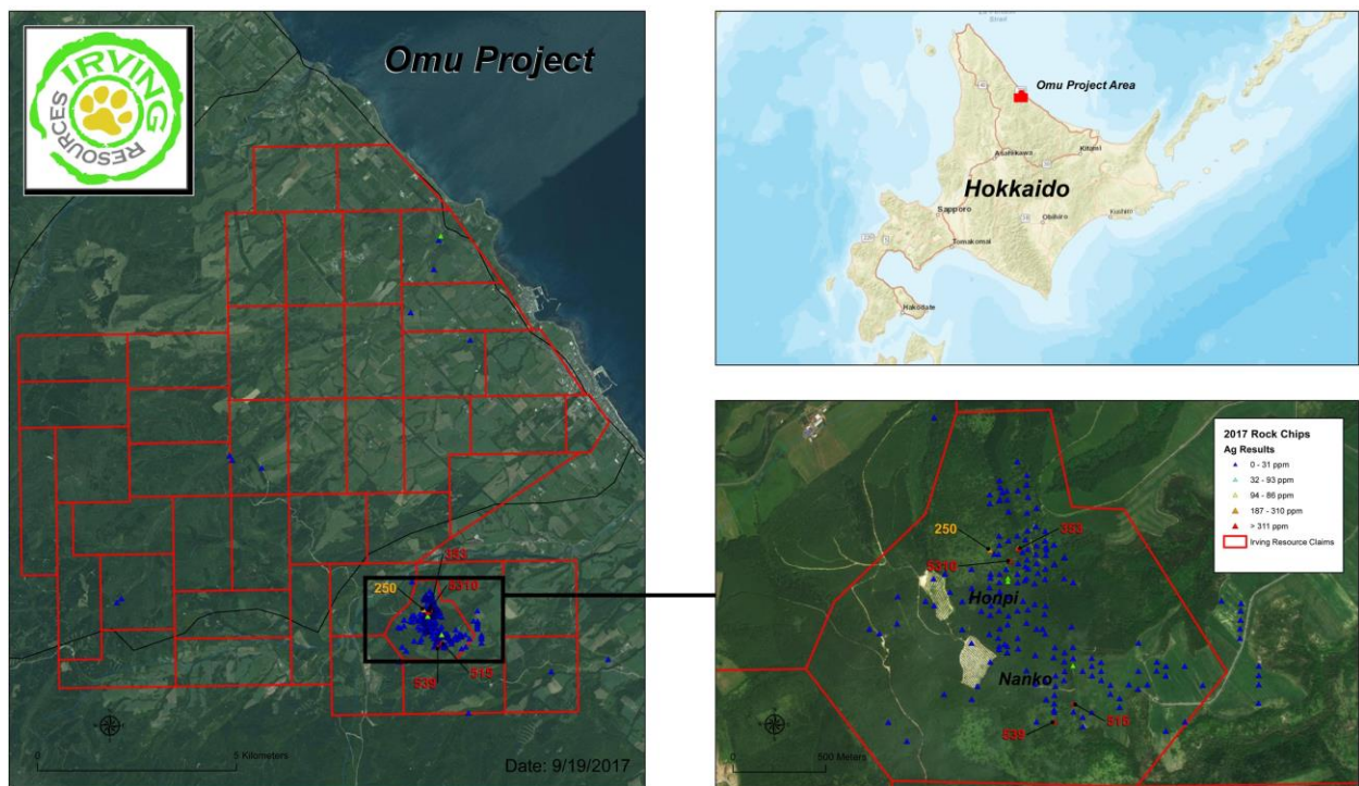
(Figure 2: Silver assays from 2017 rock chip samples.)
