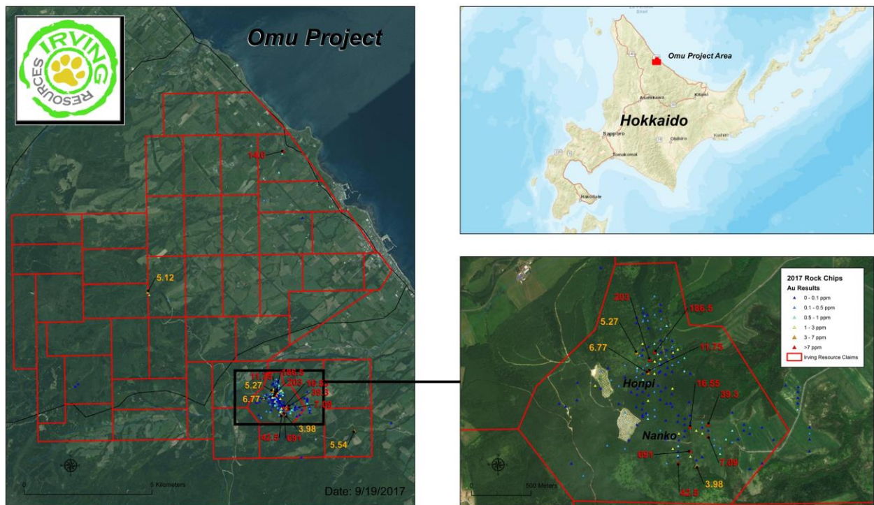
(Figure 1: Gold assays from 2017 rock chip samples.)
