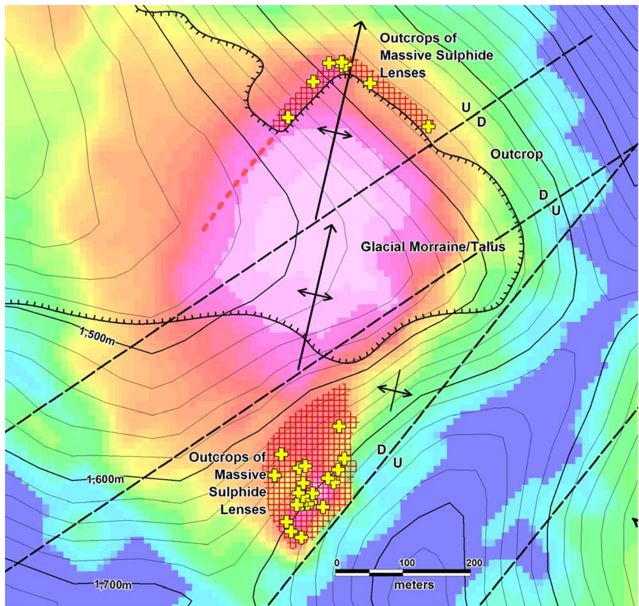
Figure 1: 7200Hz Resistivity from DIGHEM. Hot colours reflect lower resistivity, believed to be associated with selective replacement of sedimentary beds by massive pyrrhotite and chalcopyrite. Note that the resistivity correctly maps the outcropping sulphide on both sides of the central cirque. The fold structures have been mapped on the basis of measured bedding in the sediments.
