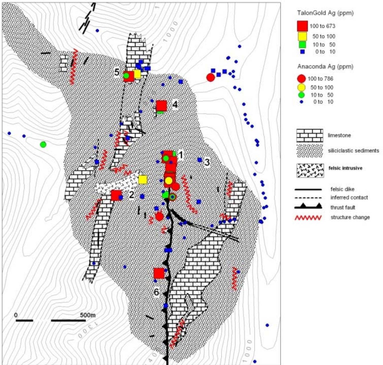
Figure 2: Geology of the Dall Prospect showing areas of copper-silver mineralization discovered to date. Area 1 is the Dall Slot, which was discovered by Anaconda. Areas 2 and 4 are the new massive sulphide zones discovered in 2008. Areas 3, 5 and 6 are areas of vein and fault breccia mineralization.
