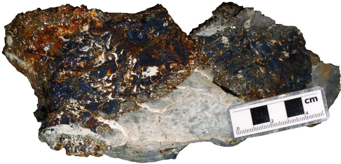
Fig. 1. Sample 016679 (UTM coords 371432E, 9316125N) Enargite-luzonite rich hydrothermal breccia matrix, with silicified dacite clasts, overprinted by kaolinite ; 8.33 g/t Au, 47.6 g/t Ag, 14.94 % Cu.
