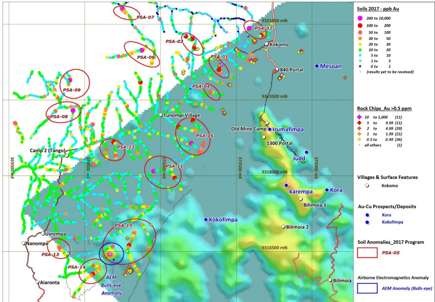
Fig. 3. Blue Lake rock chip Au assays over Au in soils (Pomasi) and AEM geophysics. Note location of prominent EM anomaly in PSA-10.
