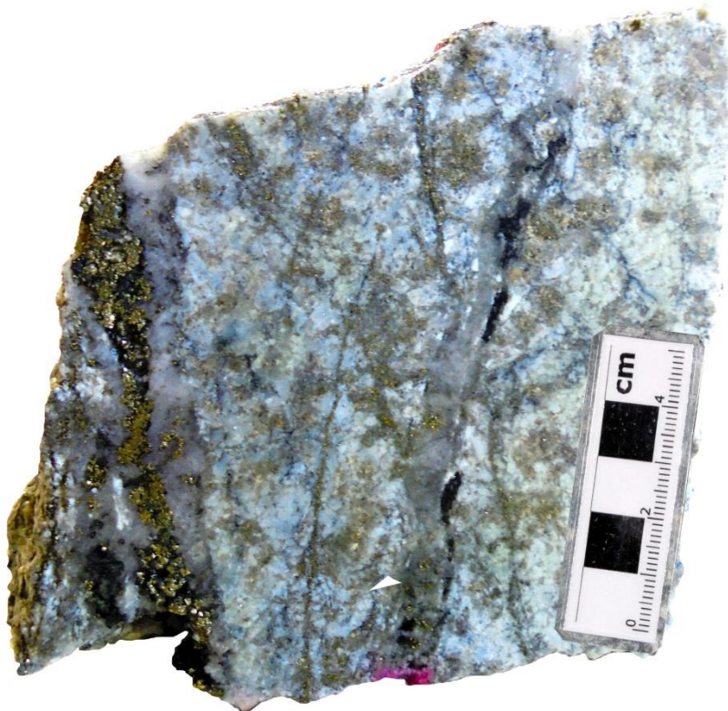
Fig. 2. Sample 021101 (UTM coords 370891E, 9316364N) Diorite with cupola textures, quartz-pyrite-chalcopyrite veins, intensely altered by pervasive dickite and disseminated pyrite; 0.14 g/t Au, 16.0 g/t Ag, 0.41 % Cu.
