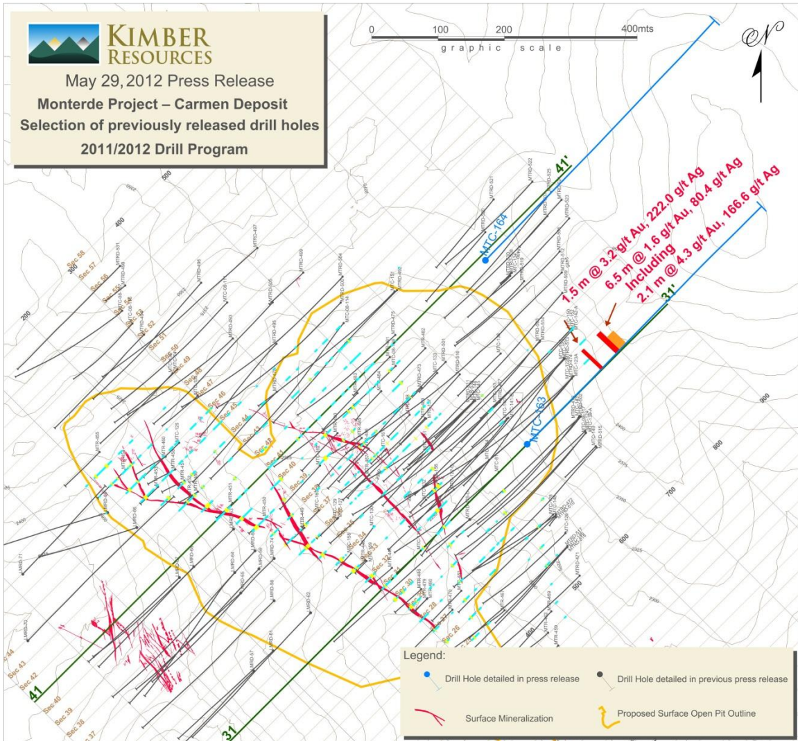
Plan view of Carmen showing the drill hole locations
