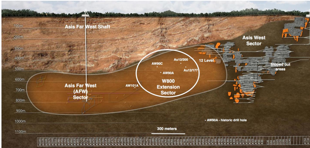
Figure 1: Kombat Mine Longitudinal Section
