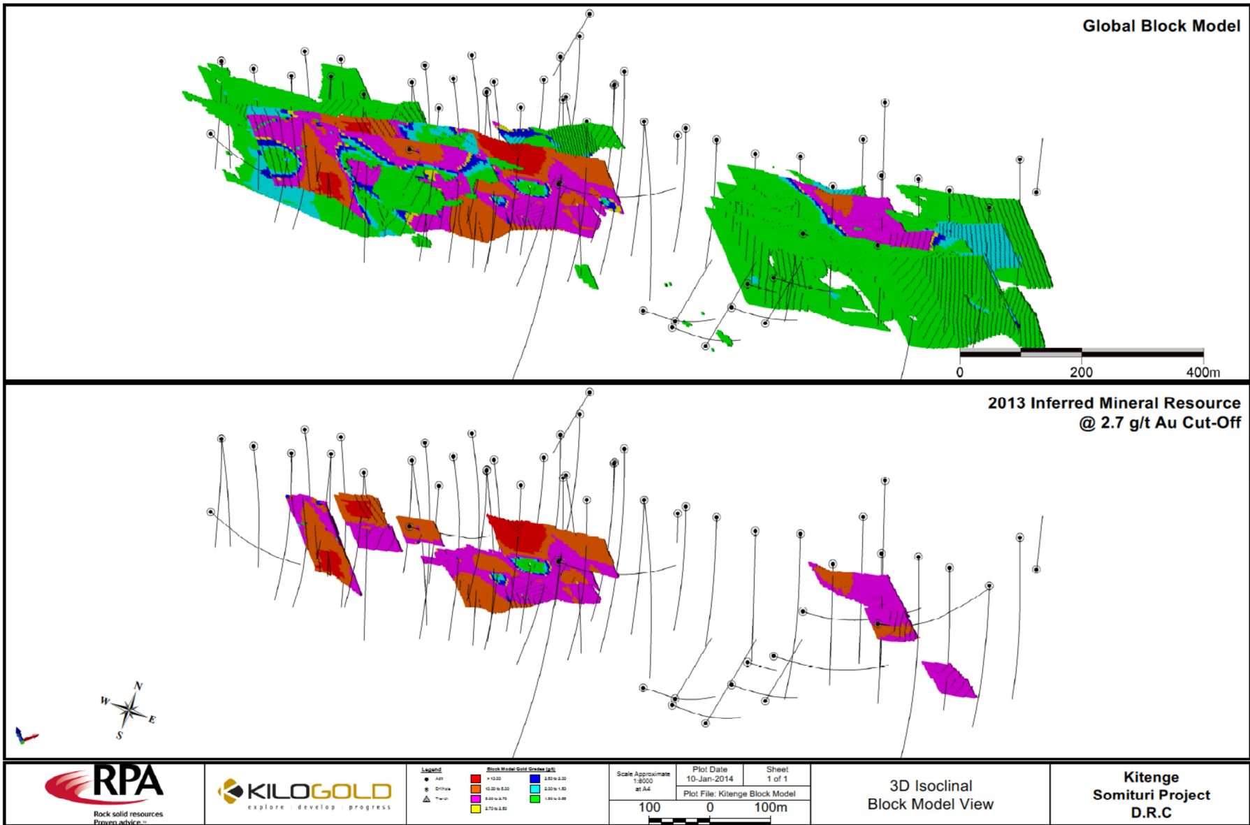
Figure 3: Kitenge Inferred Mineral Resources at a 2.70 g/t Au cut-off grade
