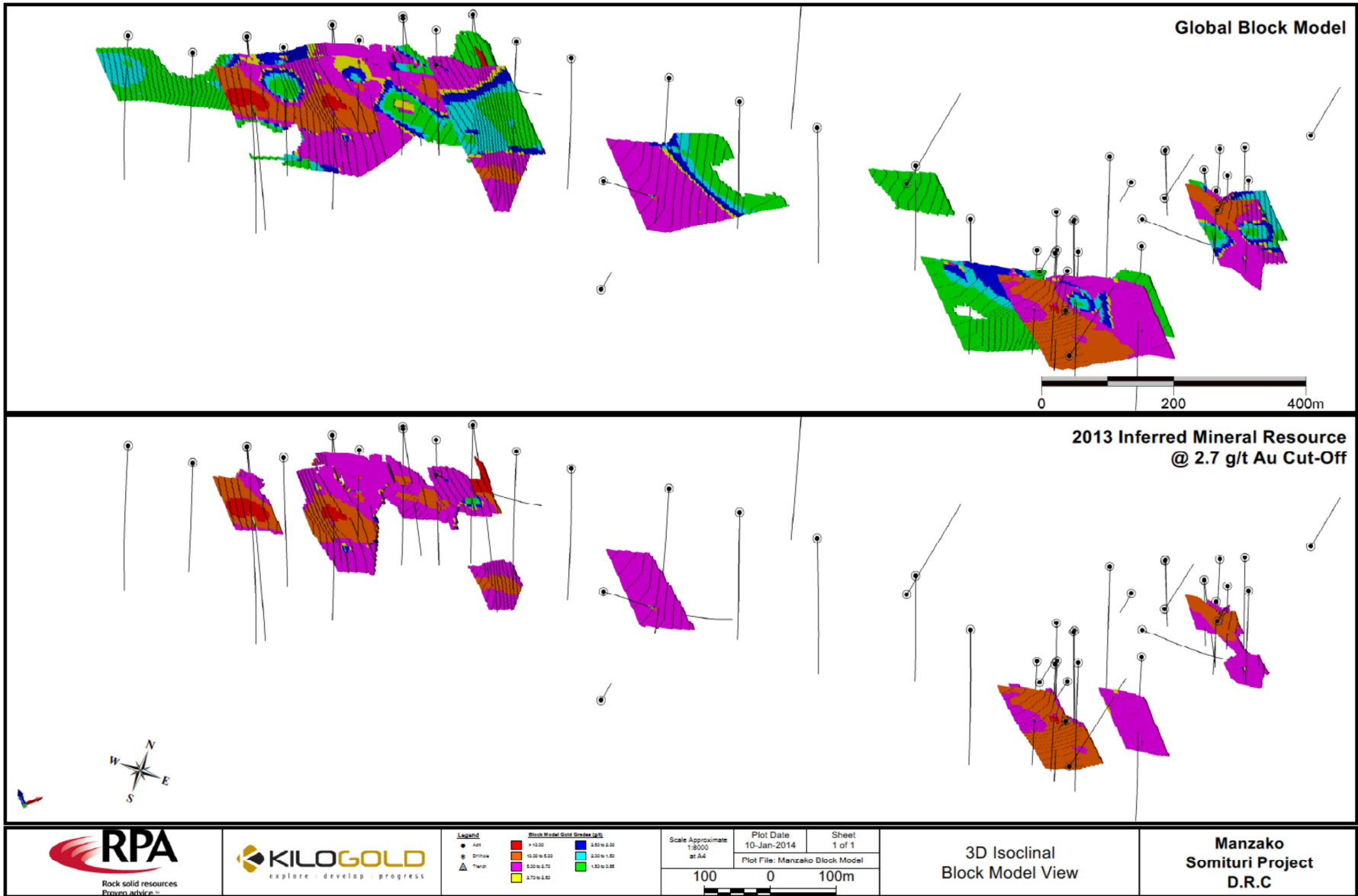
Figure 4: Manzako Inferred Resources at a 2.70 g/t Au cut-off grade
