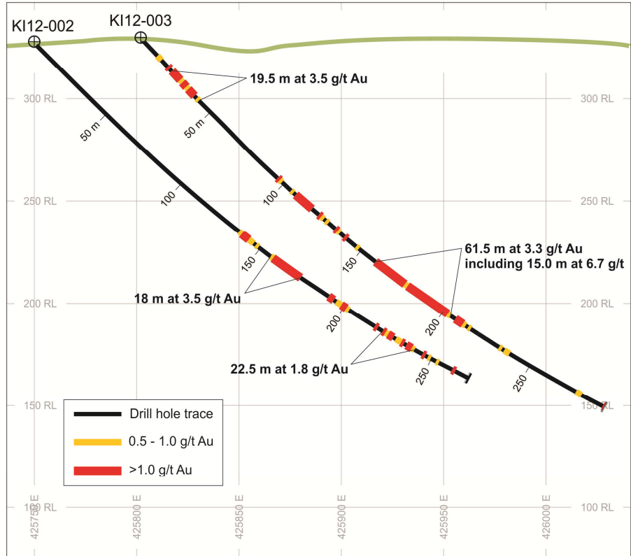
Figure 3: KI12-002 and KI12-003 cross section.
