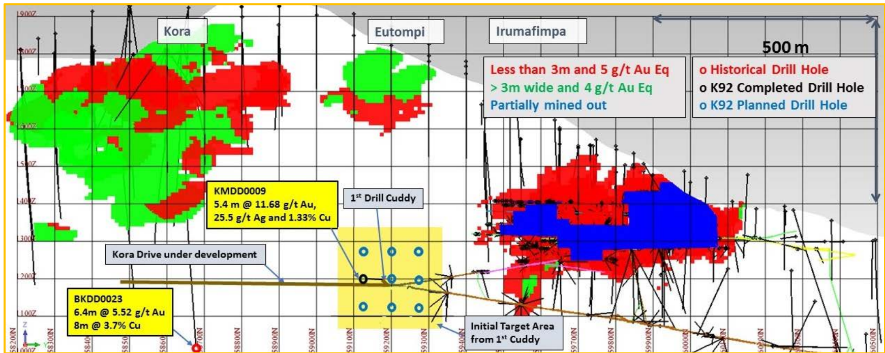
Figure 1 Long Section through the Irumafimpa and Kora Deposits
