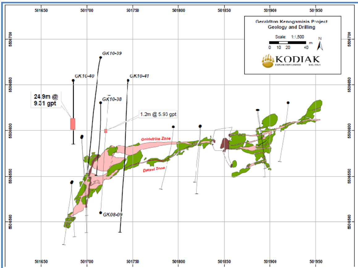
Drill hole location map, GK target area, West Geraldton Project. The gold mineralization seen in drill hole GK10-40 is open down-dip, to the west and down plunge to the east.
