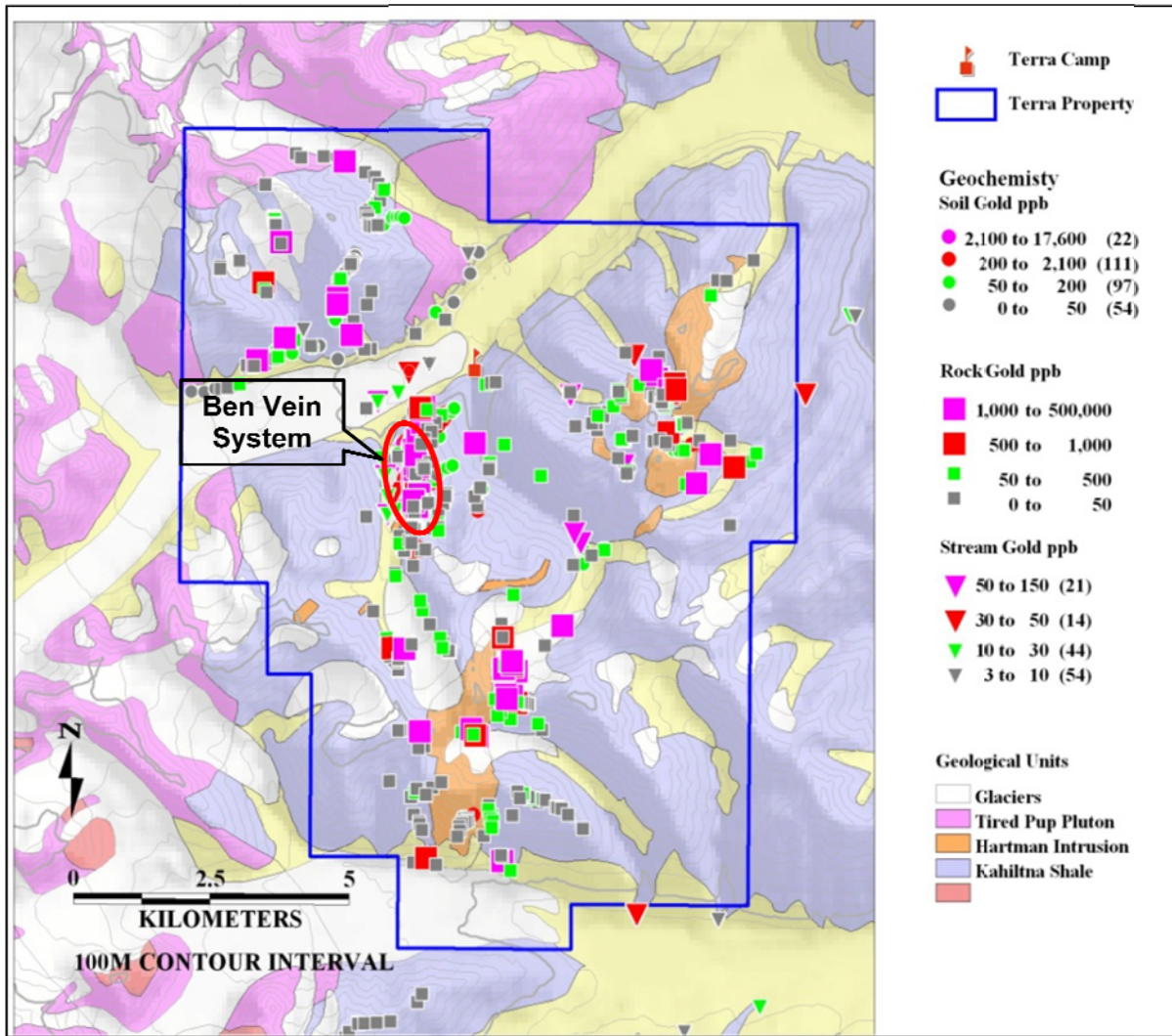
Figure 1: Terra project area map showing major geologic units and surface gold mineralization. The Ben Vein system is highlighted in the center of the map, and will be the focus of the 2011 development program.
