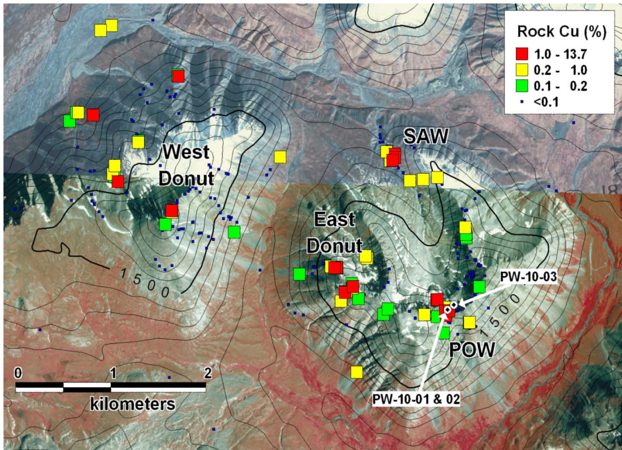
Figure 1: Air photo base showing the locations of copper mineralization in the vicinity of the POW Prospect. Drill hole PW-10-03 was lost prior to reaching its target depth.
