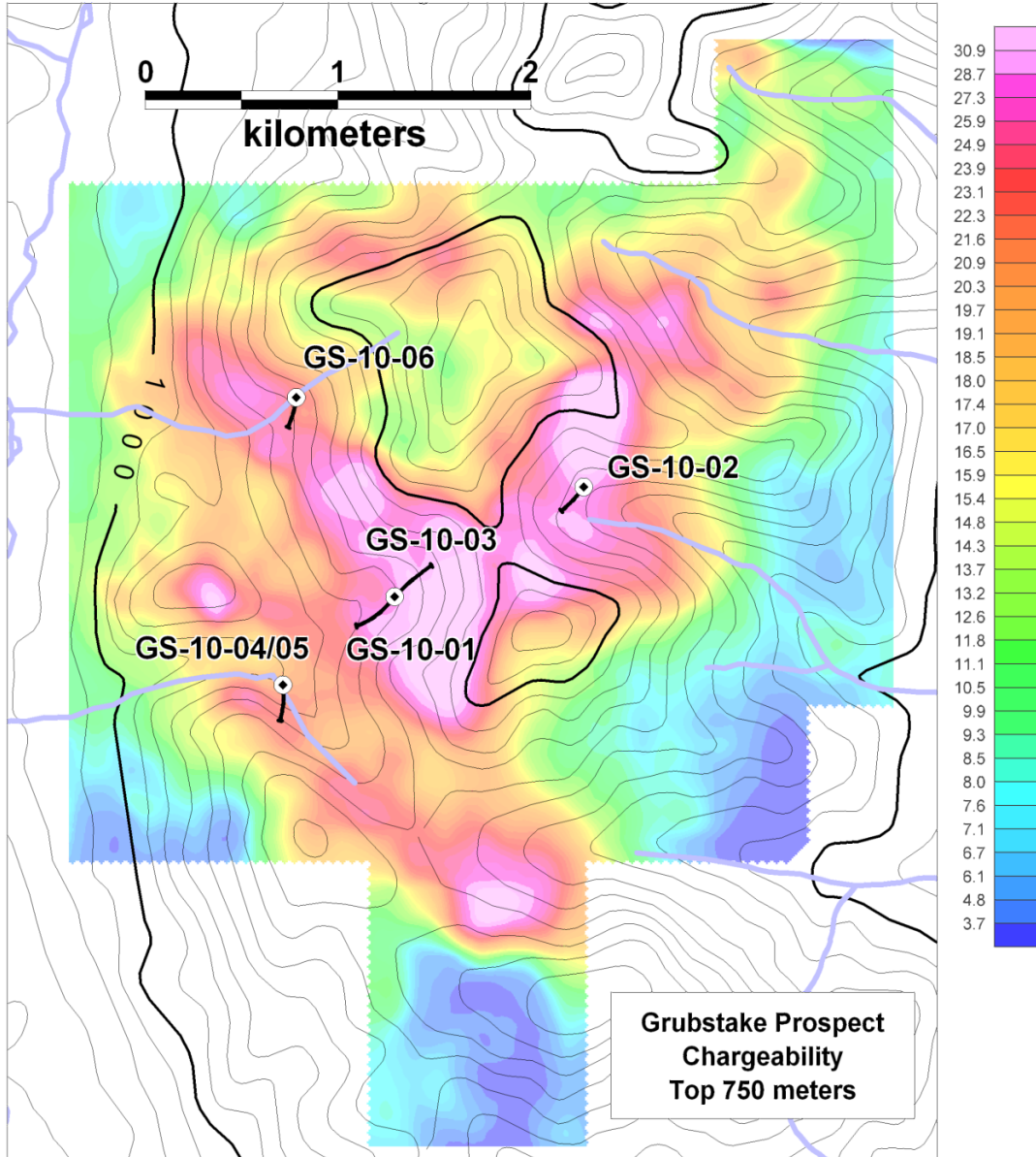
Figure 2: Ground IP chargeability map of the Grubstake target with completed drill holes (results pending). Topographic contour is 50 meters.
