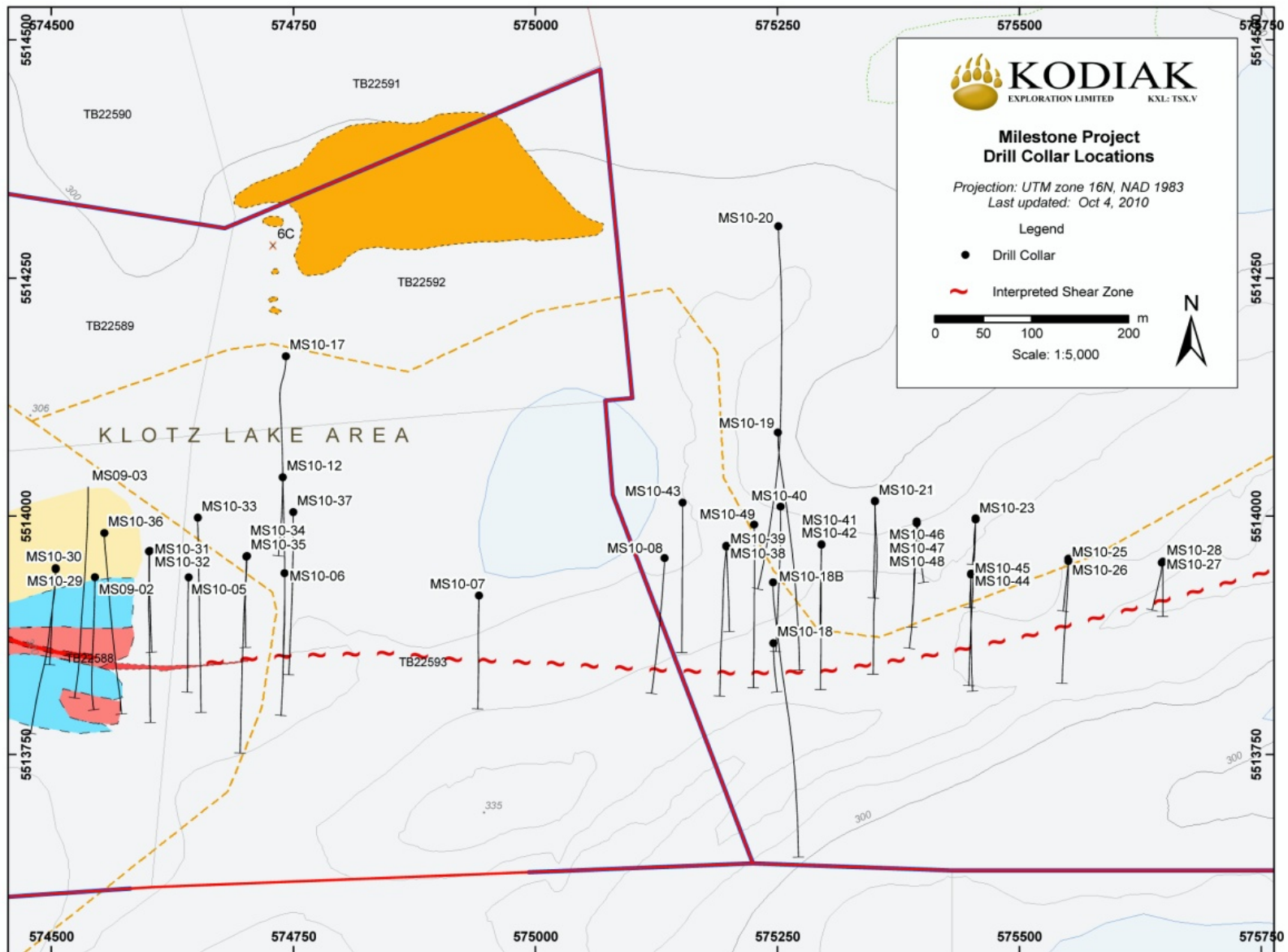
Drill hole location map, Milestone Project, Ontario
