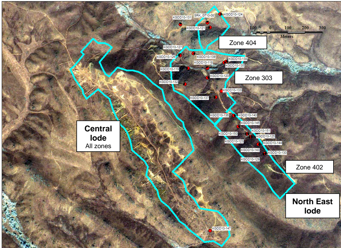
Figure 1. Location of the 2010 infill drillholes relative to the mineral zones in the Central and North East lodges at the Karchiga deposit. The projection of the Central and North East lodges to surface is shown according to the March 22, 2010 mineral resource statement (Table 1).
