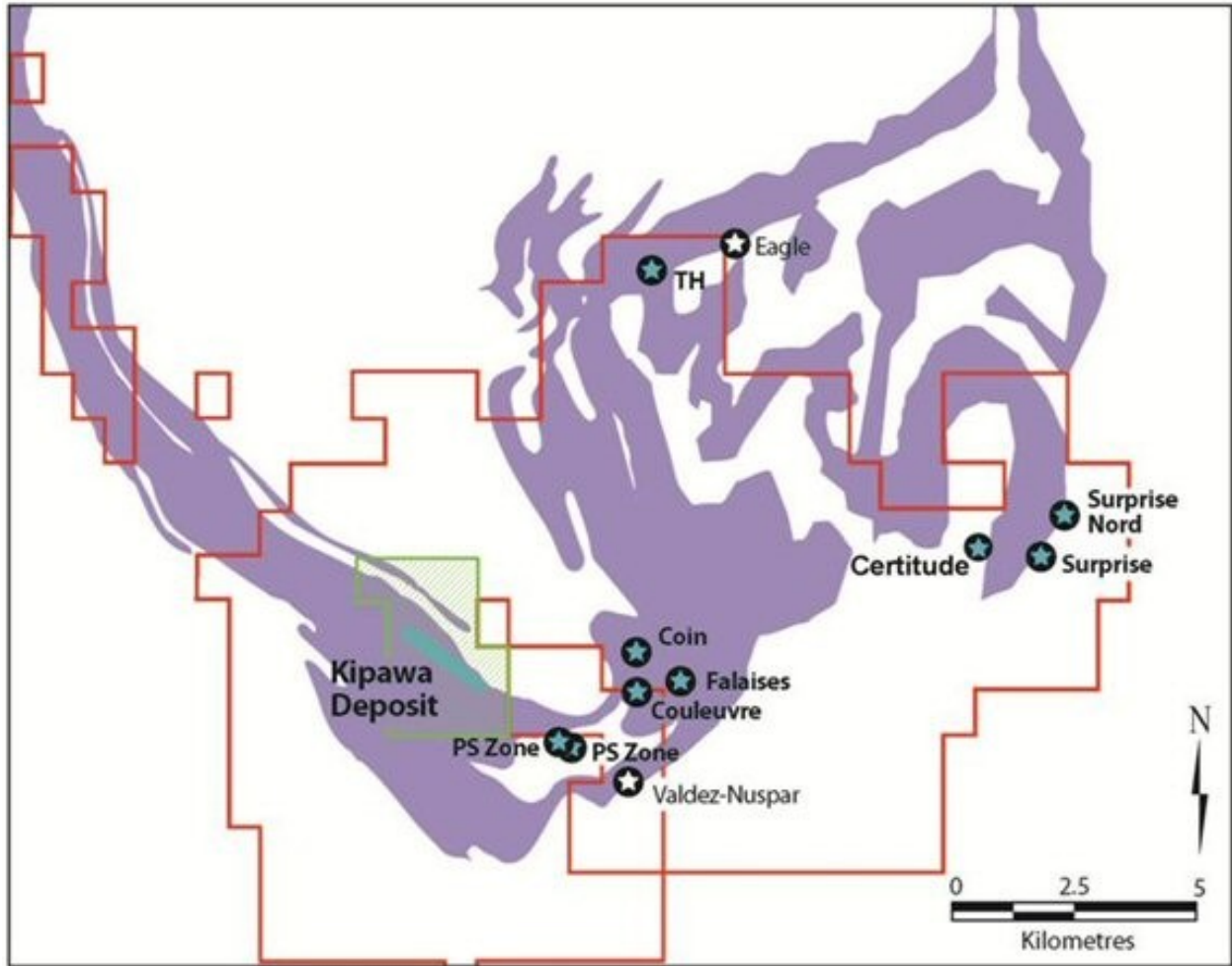
Figure 1. Matamec: Kipawa deposit and Zeus property areas (Green = Matamec-Toyota Tsusho MOU: Kipawa deposit) (Red = Matamec: Zeus property with showings in blue stars) (Purple = Kipawa Alkalic Complex)
