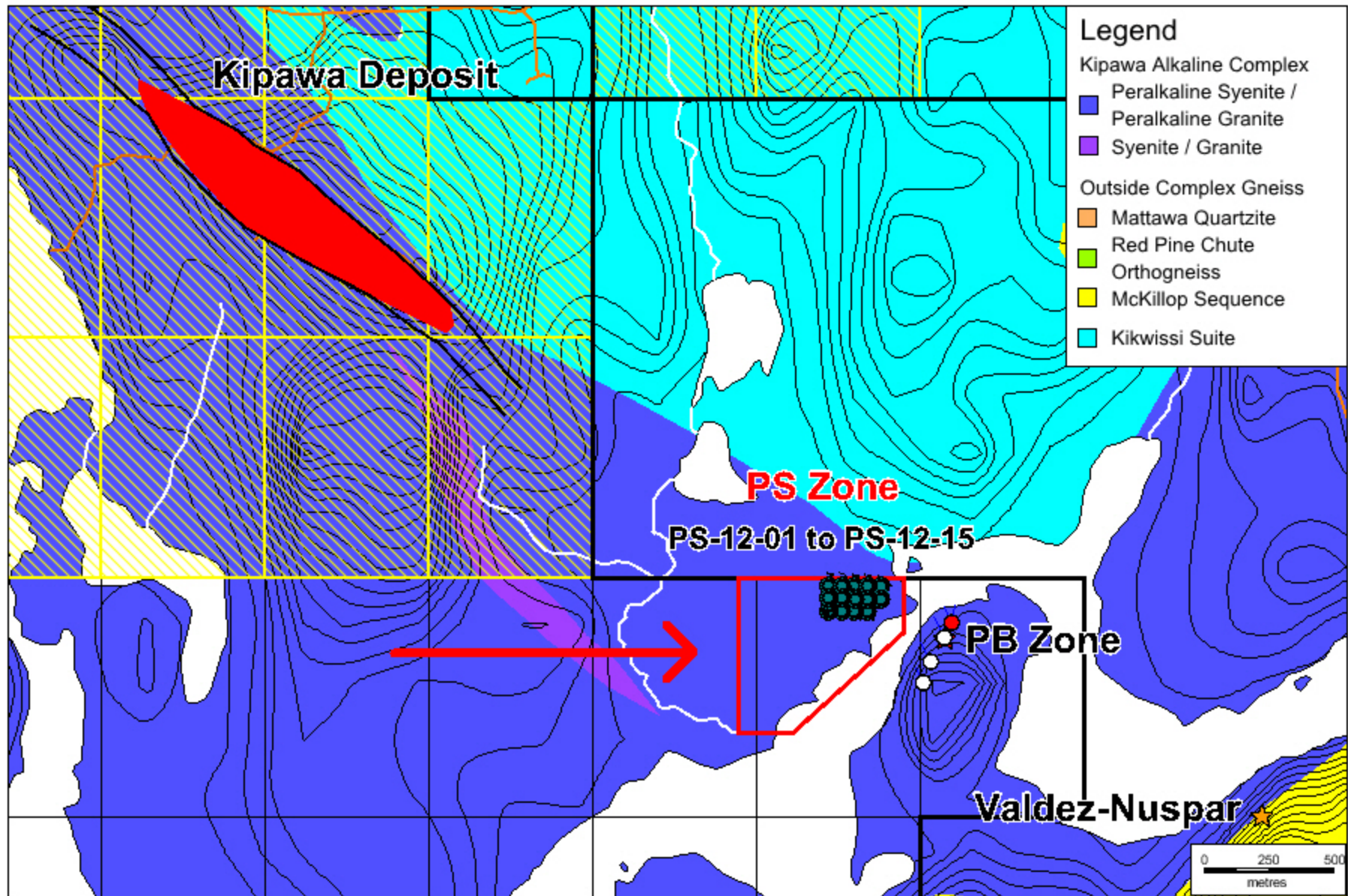
Figure 1: Drill holes location on PS Zone, Matamec Explorations inc. Holes drilled by Unocal on PB zone in red (mineralized hole) and white (unmineralized hole). Joint venture claims in yellow.
