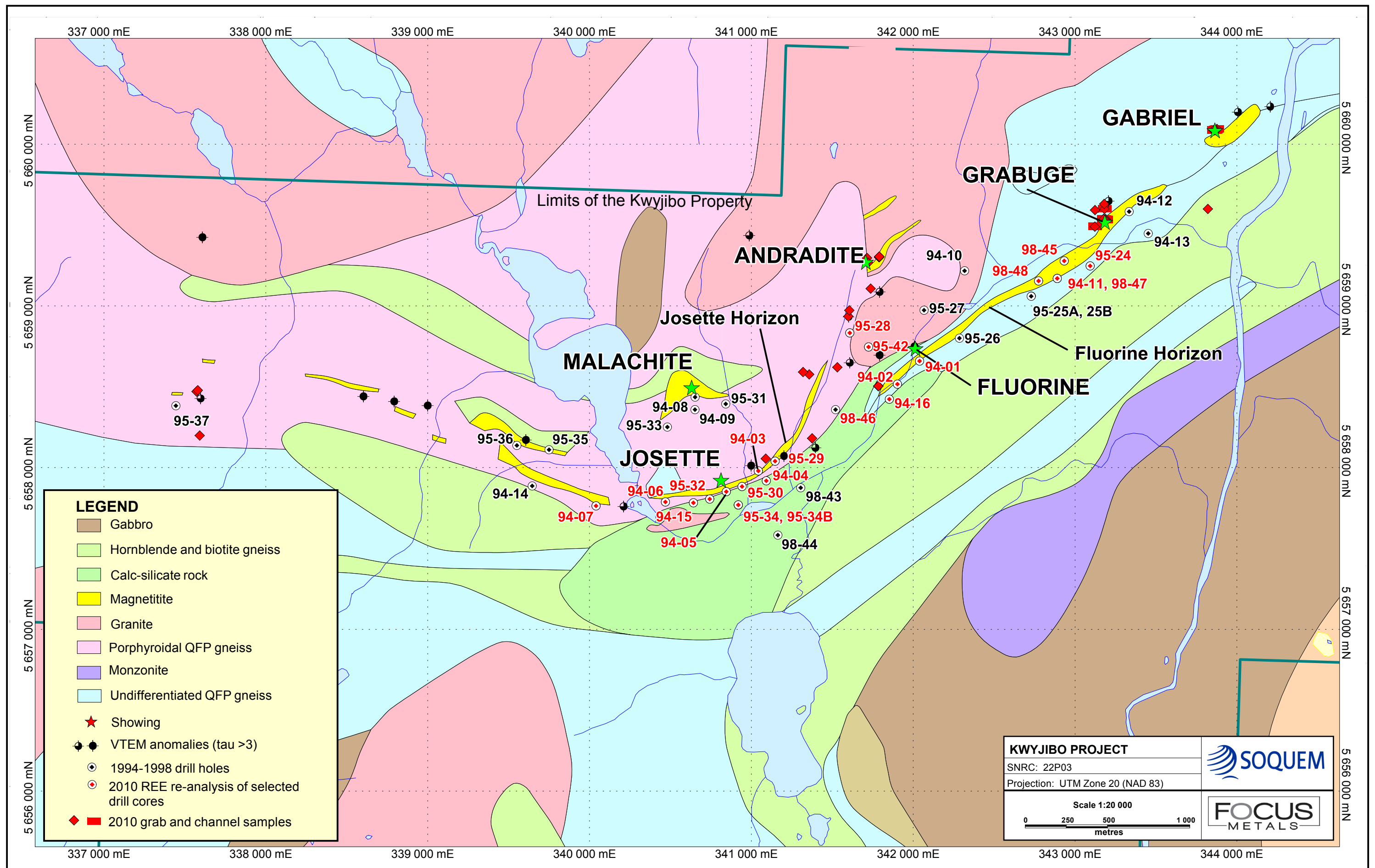
Figure 1. Location of the drill holes (in red) of the fall 2010 re-analysis REE program of drill cores. 2010 grab and channel samples and 2006 VTEM anomalies on the geological map of the Kwijibo Property.
