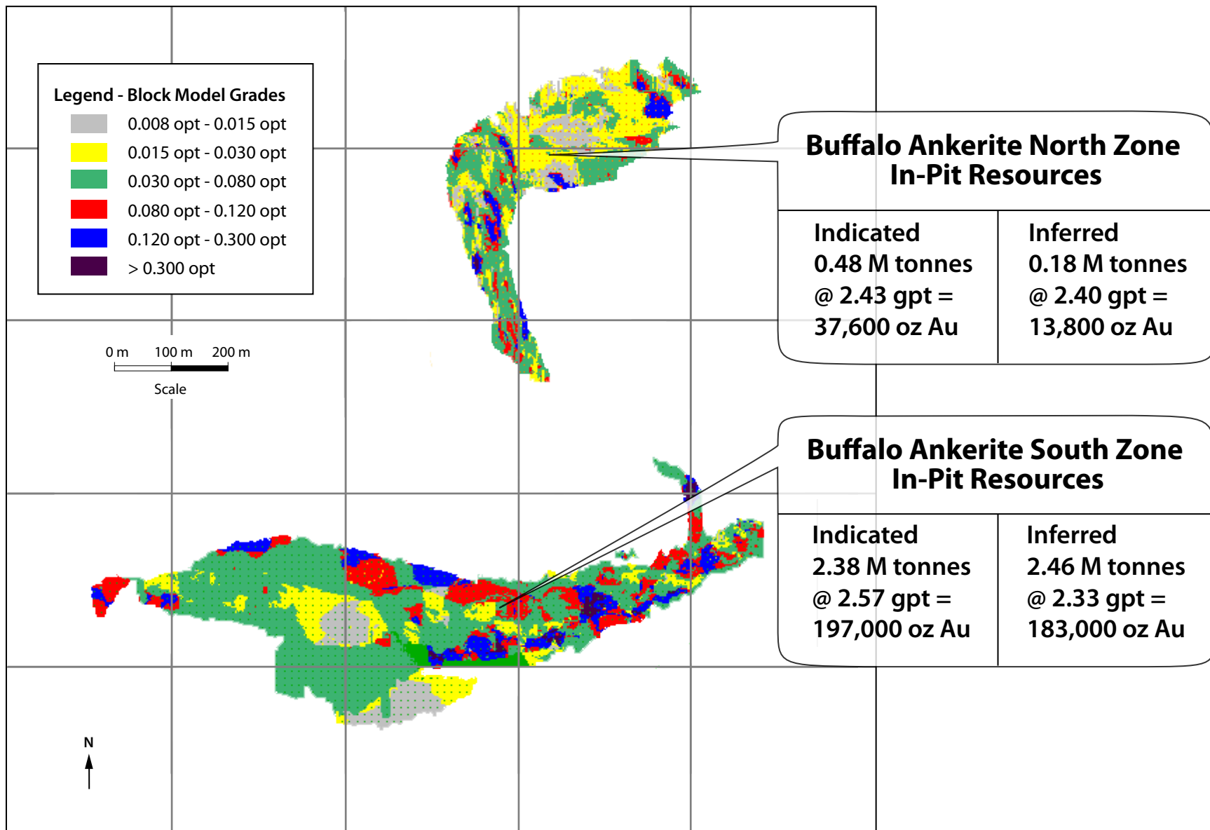
Figure 1. Buffalo Ankerite In-Pit Resources North and South Zones With Color Grade Blocks (Surface Plan Map)
