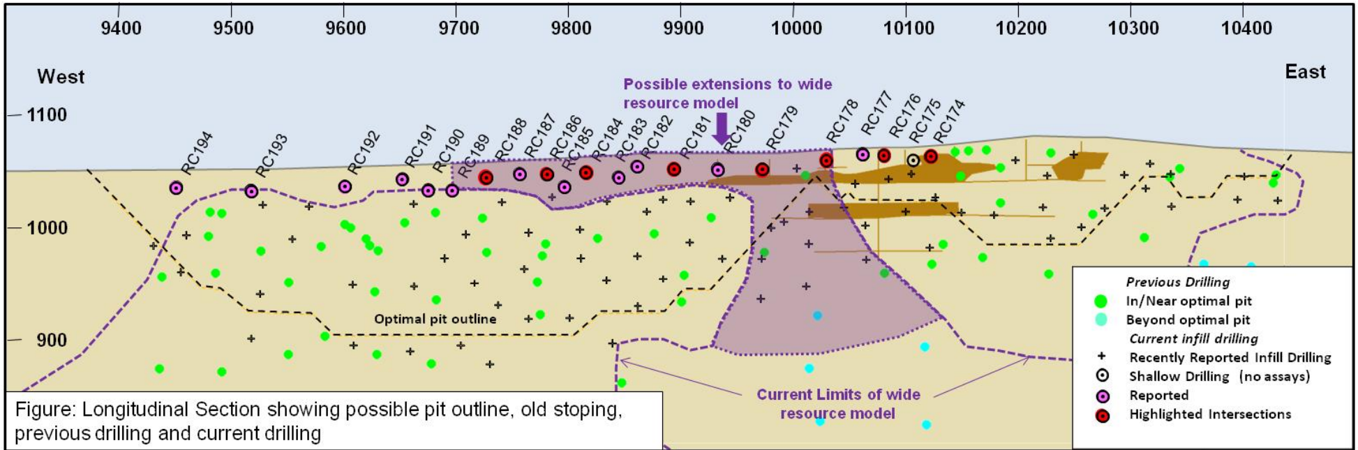
Figure 1: Matala deposit – Longitudinal Section showing of drilling results (Note the drill hole names have been shortened for plotting)
