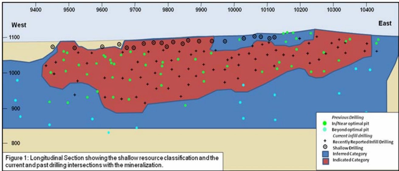
Figure 1: Matala deposit – Longitudinal Section Mineral Resource Categories for the shallow resource.
