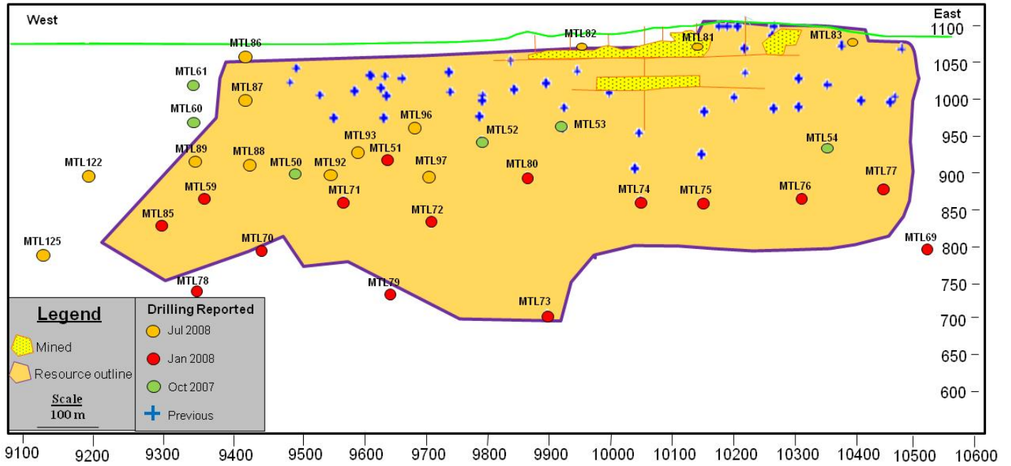
Figure 1: Longitudinal section of Matala deposit showing drill hole intersection points
