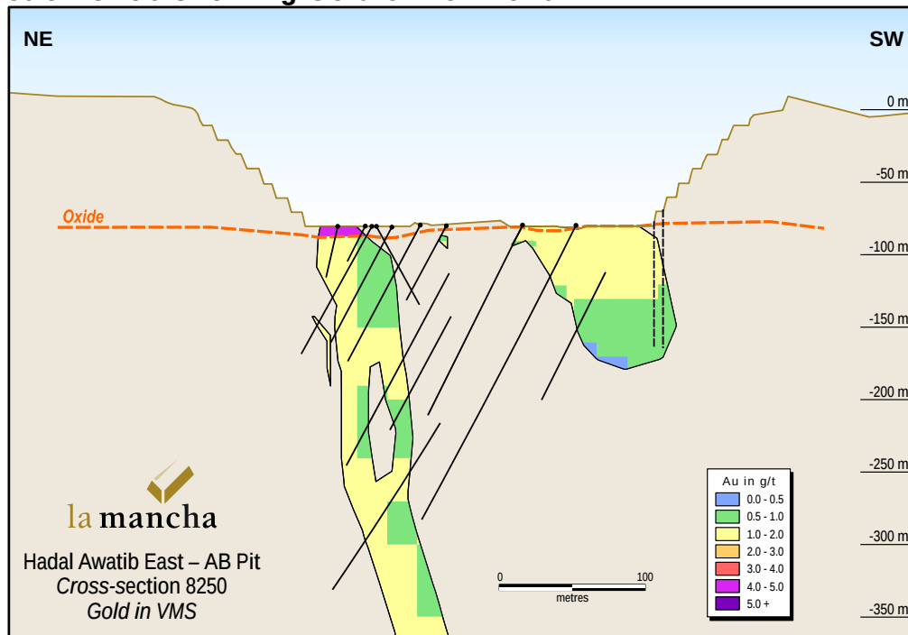
Figure 2a Cross-section 8250 showing Gold enrichment
