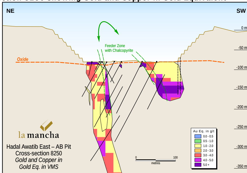
Figure 2b Cross-section 8250 showing Gold and Copper in Gold Equivalent
