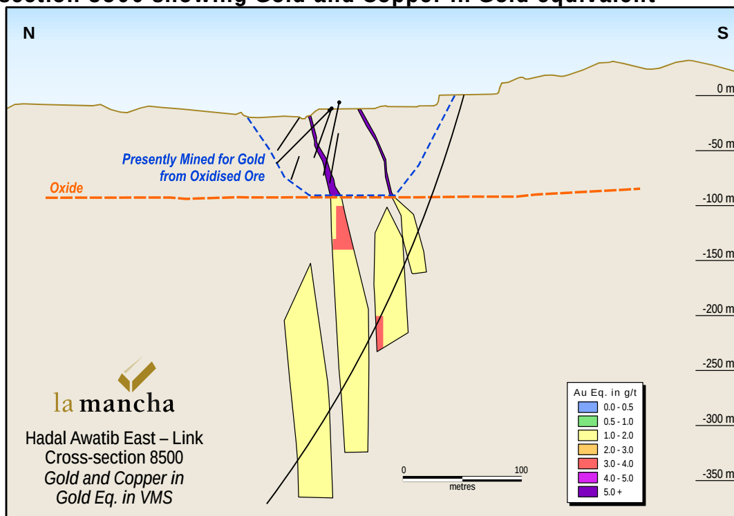
Figure 3b Cross-section 8500 showing Gold and Copper in Gold equivalent
