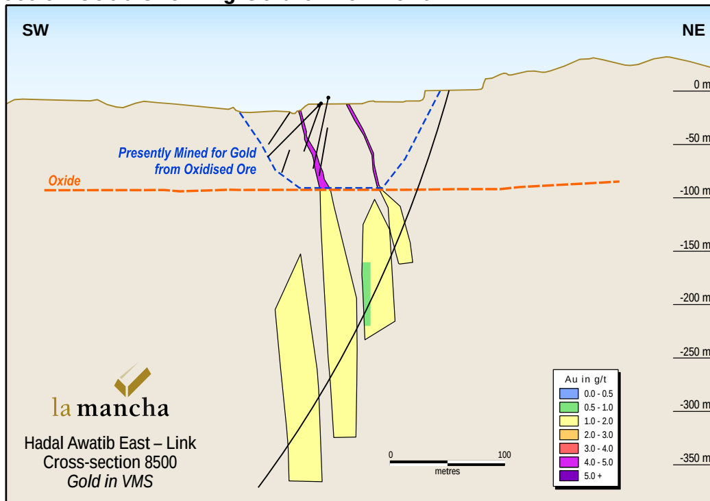
Figure 3a Cross-section 8500 showing Gold enrichment
