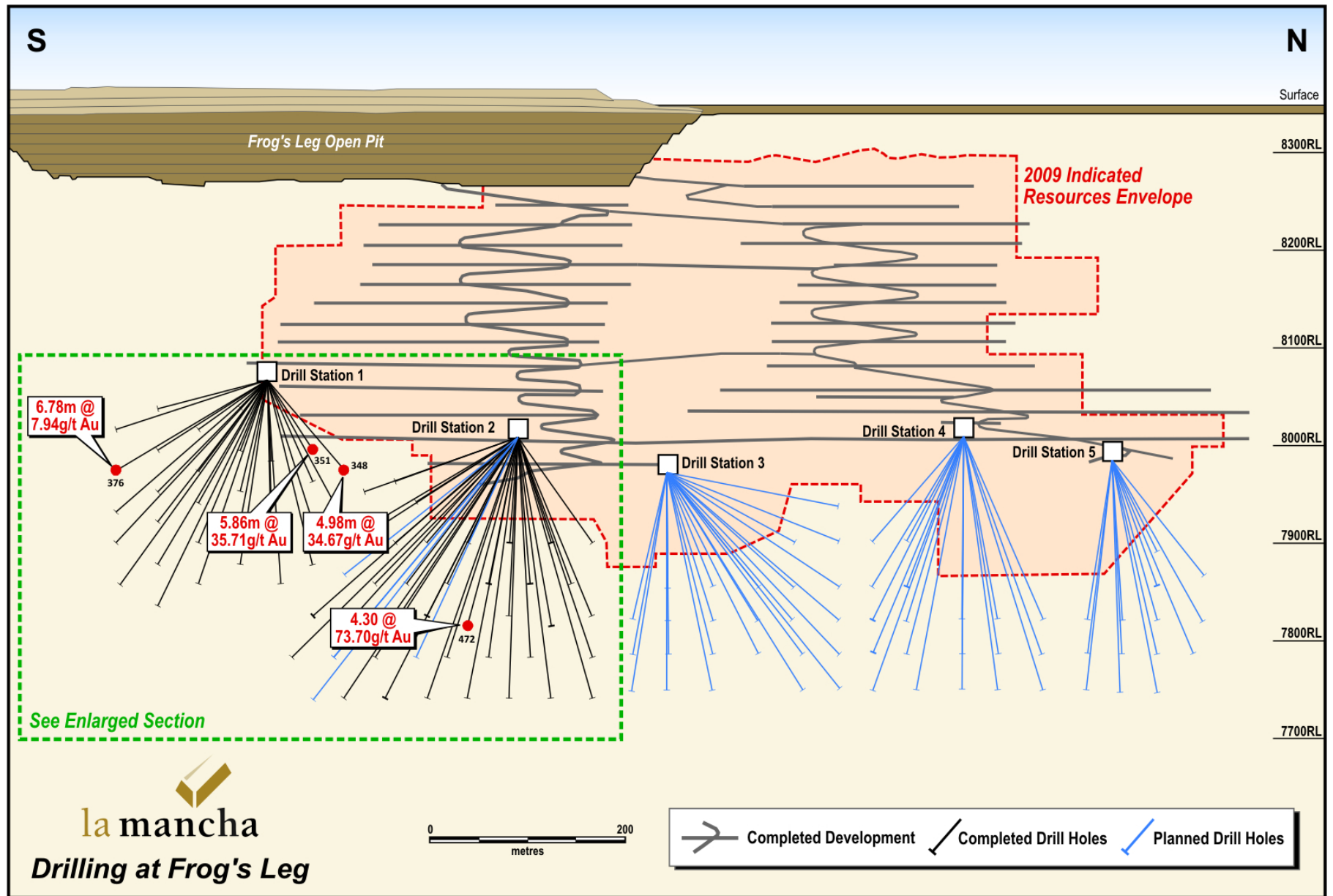
Figure 1: Cross-section
