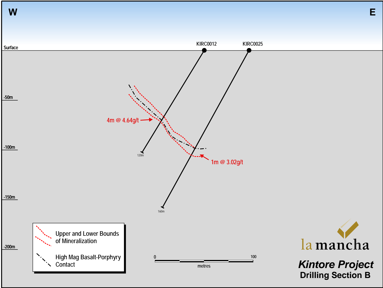
Figures 3b : Cross-section
