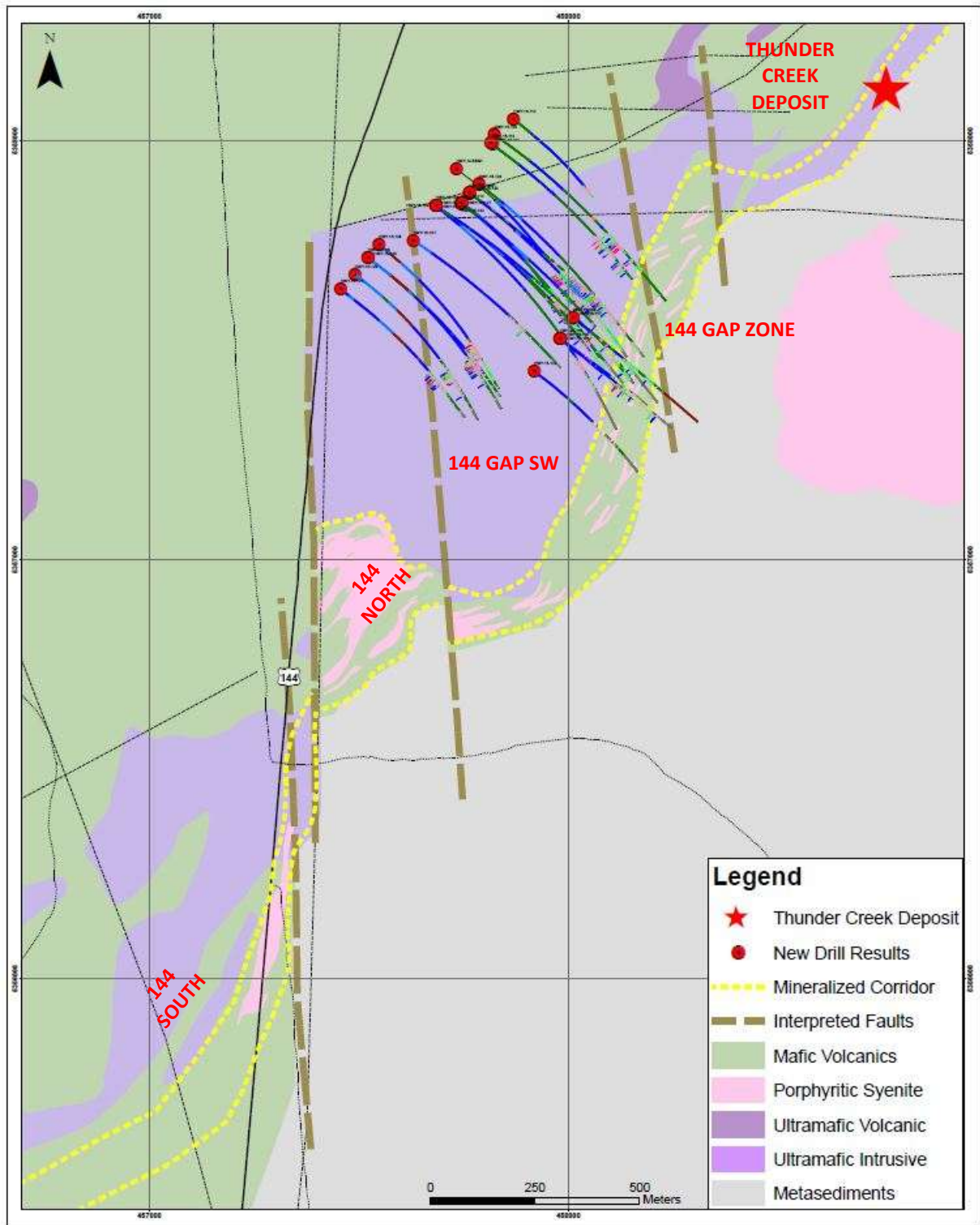
Figure 2. 144 Trend Surface Geology Plan – New Drill Holes (Projected Vertically to Surface)
