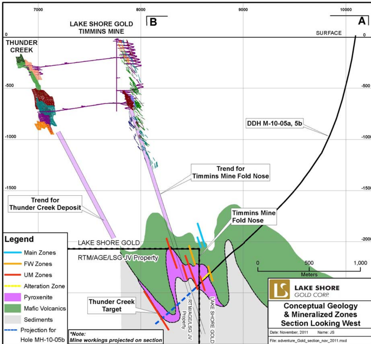
Figure 1. Cross Section
