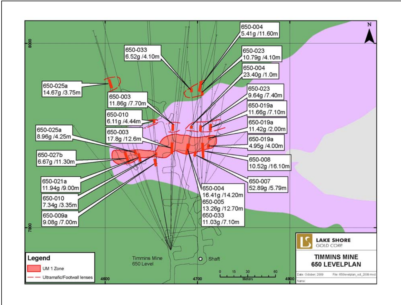
Figure 1. Plan View
