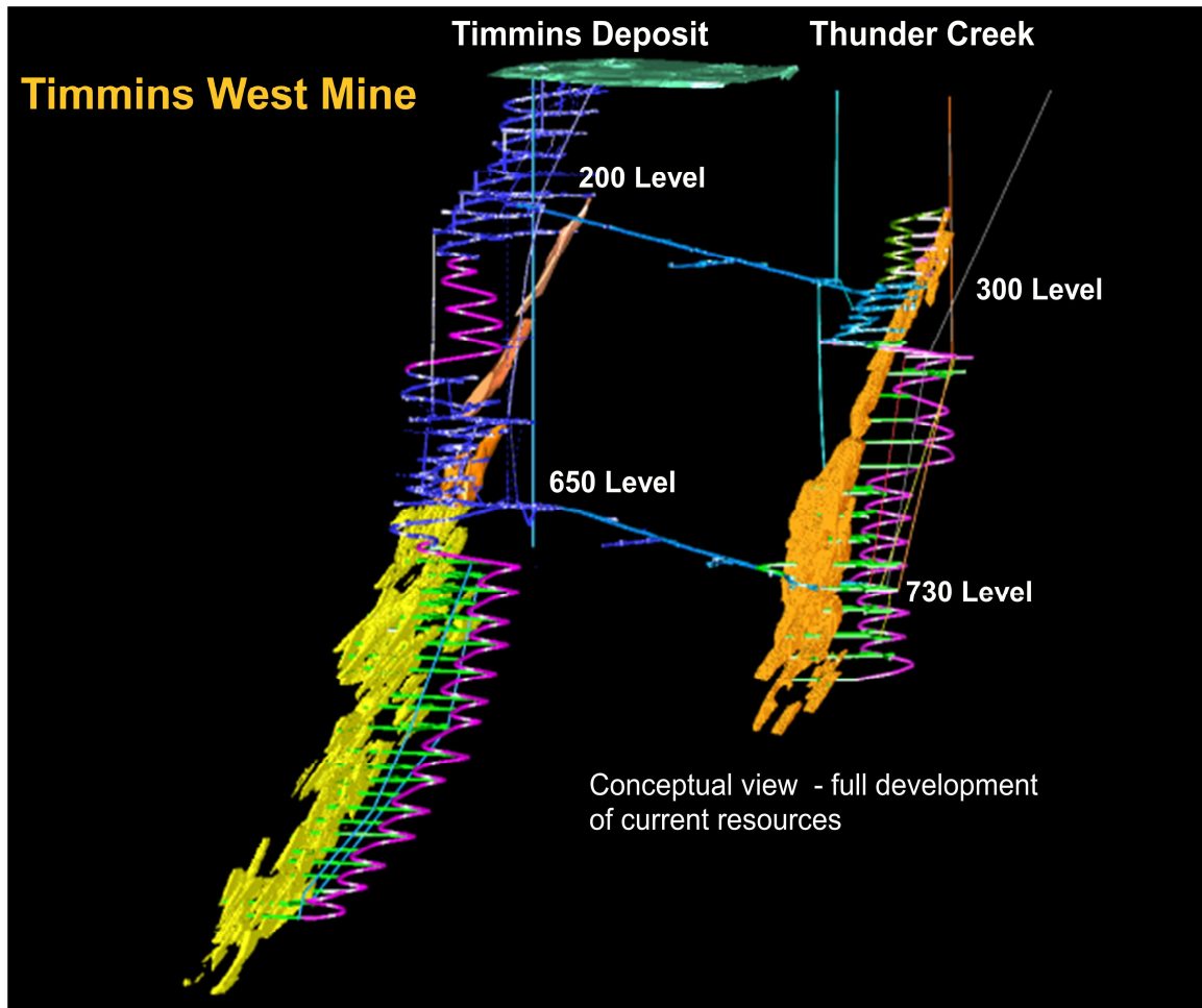
Figure 1. Conceptual View – Timmins West Mine Development
