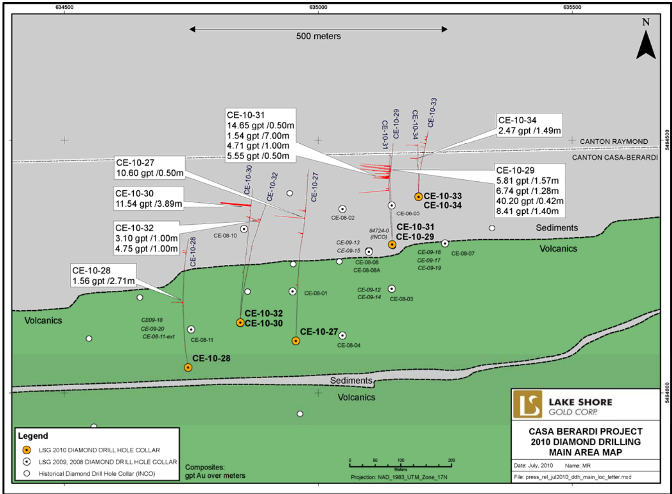
Figure 1. Plan View
