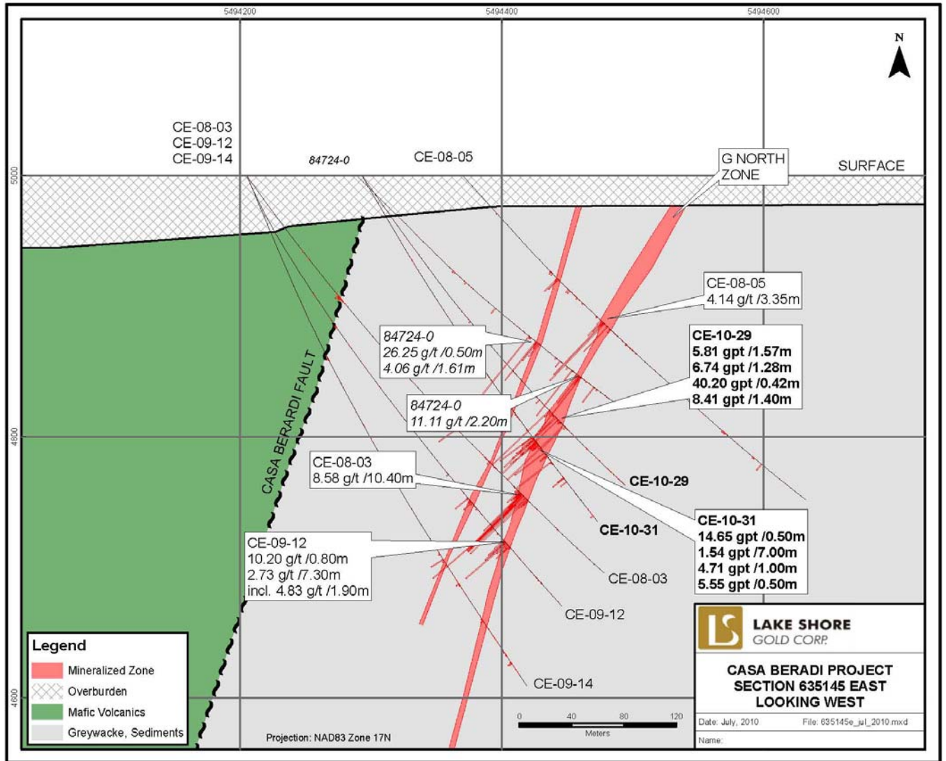
Figure 2. Cross Section 635145
