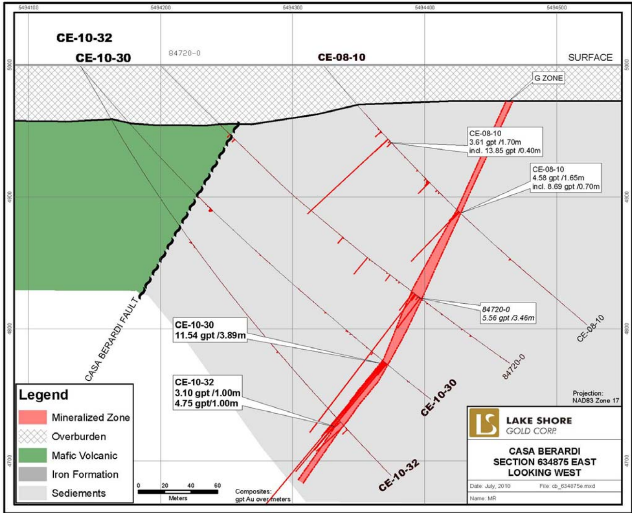
Figure 3: Cross Section 634875
