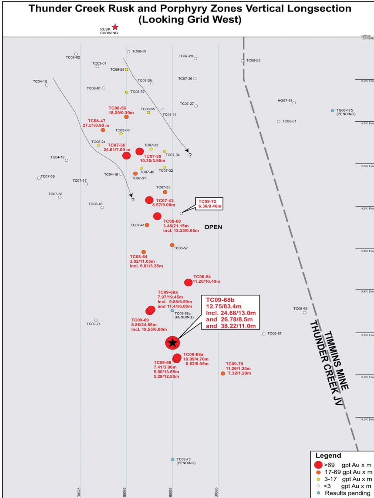
Figure 2. Long Section
