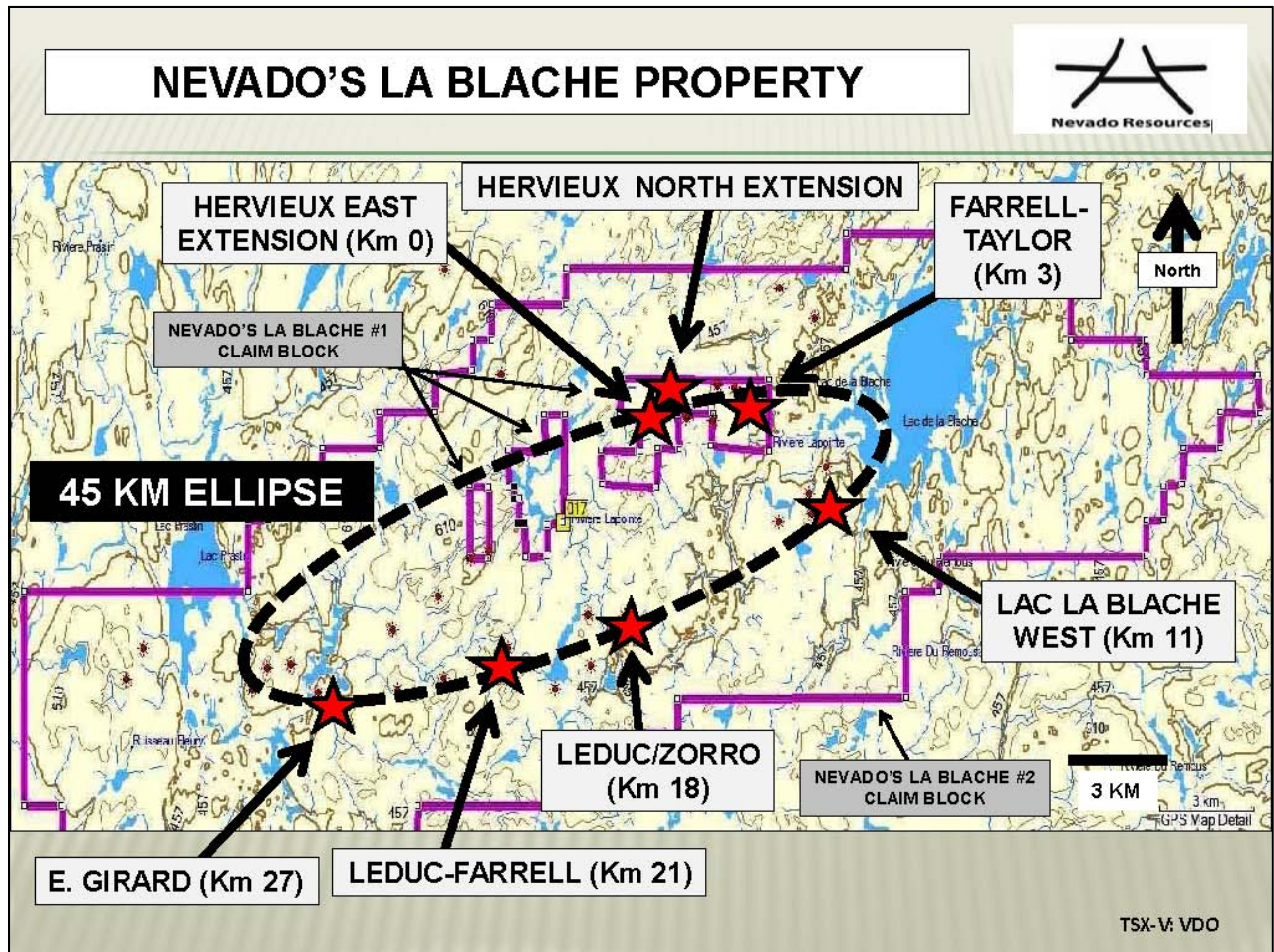
Figure 1: Schematic location map outlining the 45 kilometre perimeter of the La Blache Ring of Iron-Titanium-Vanadium, an 18 kilometres by 10 kilometres ellipse that hosts the seven (7) recently discovered magnetite-ilmenite occurrences on NEVADO's La Blache Property (Quebec).
