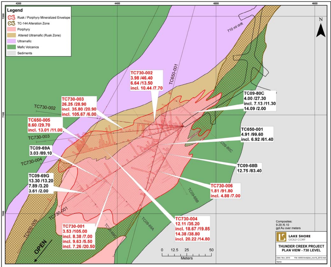
Figure 2. Plan View (Drilling)
