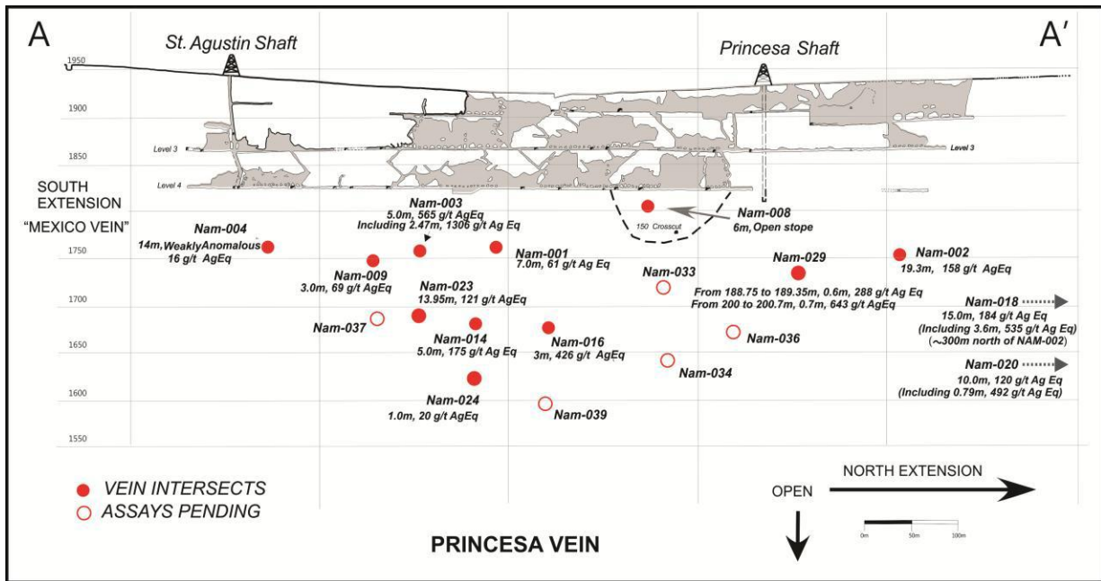
2d View of Long section with Peirce points from 2011 drilling
