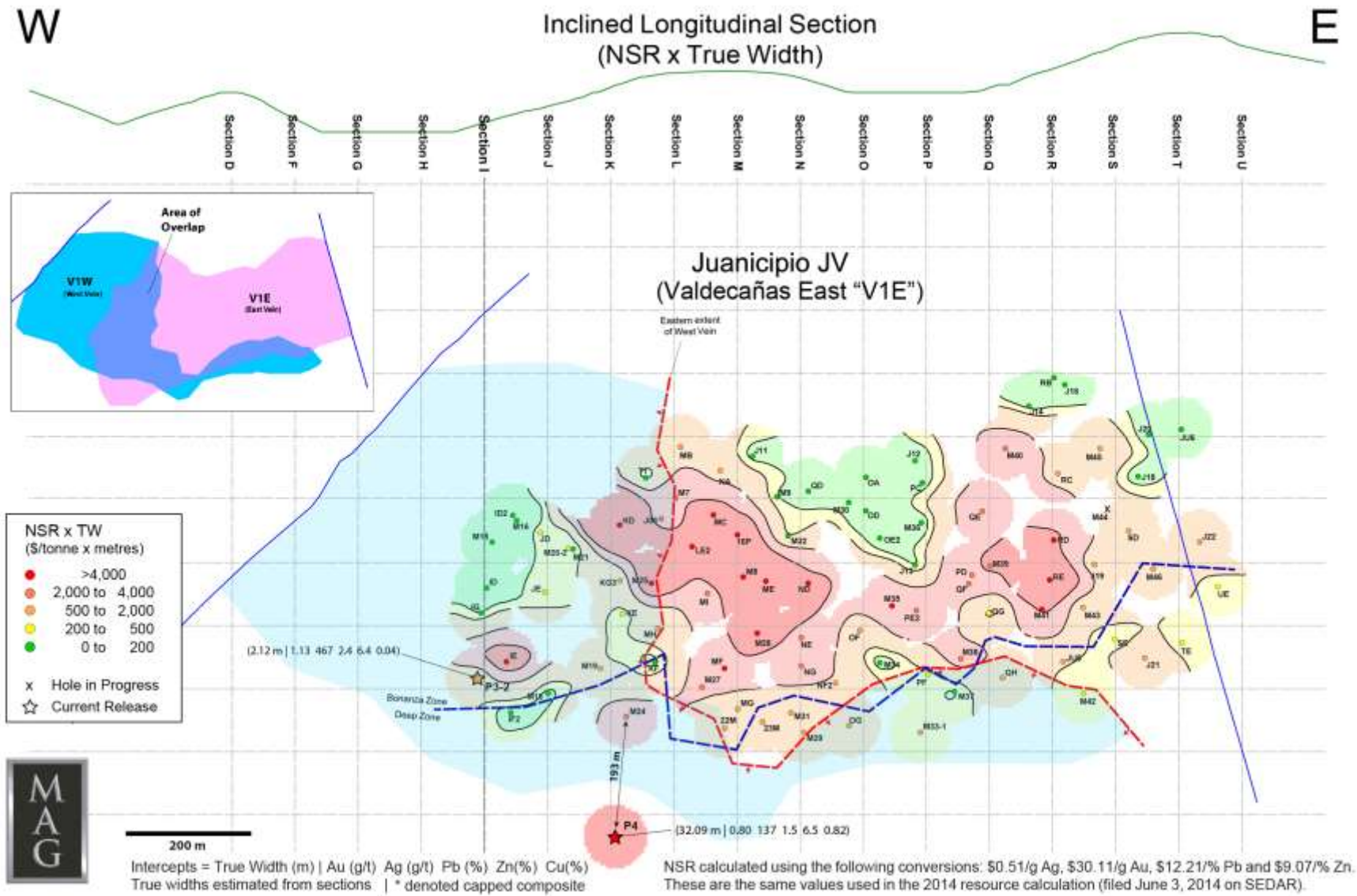
Figure 3: Minera Juancipio, Valdecañas East – Longitudinal Section
