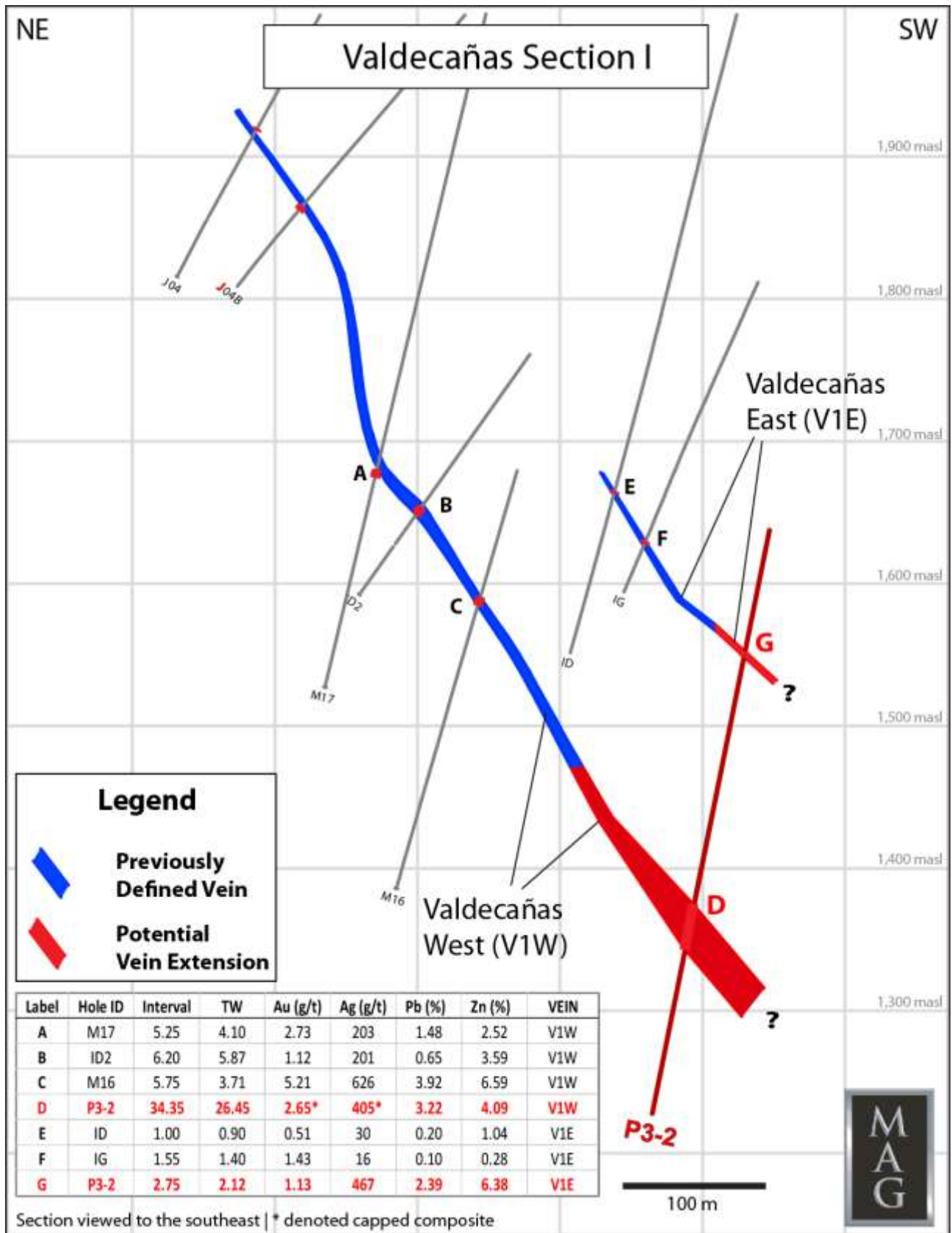
Figure 1: Minera Juancipio, Valdecañas Veins - Cross Section
