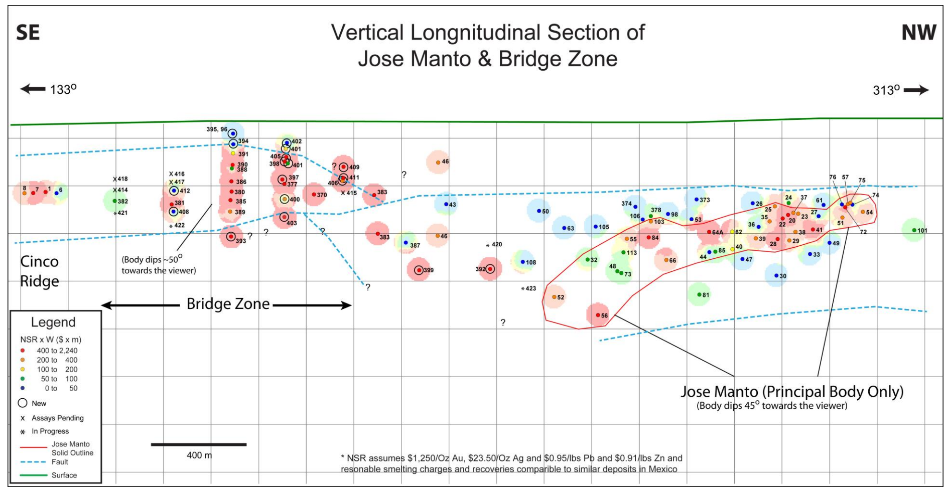
Figure Three: Longitudinal Section
