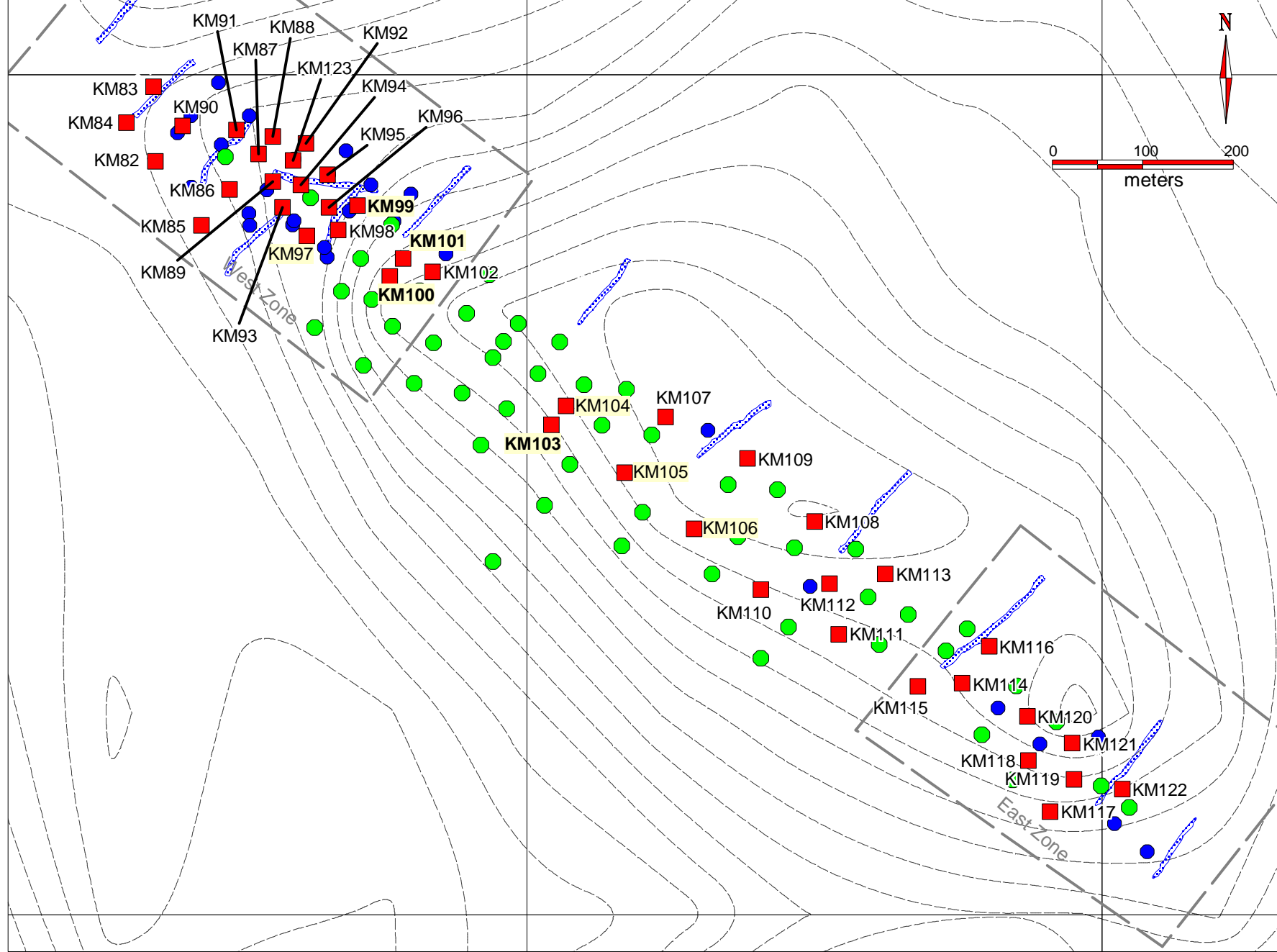
Fig 1. Matamec 2010-2011 drilling campaign, Kipawa deposit
