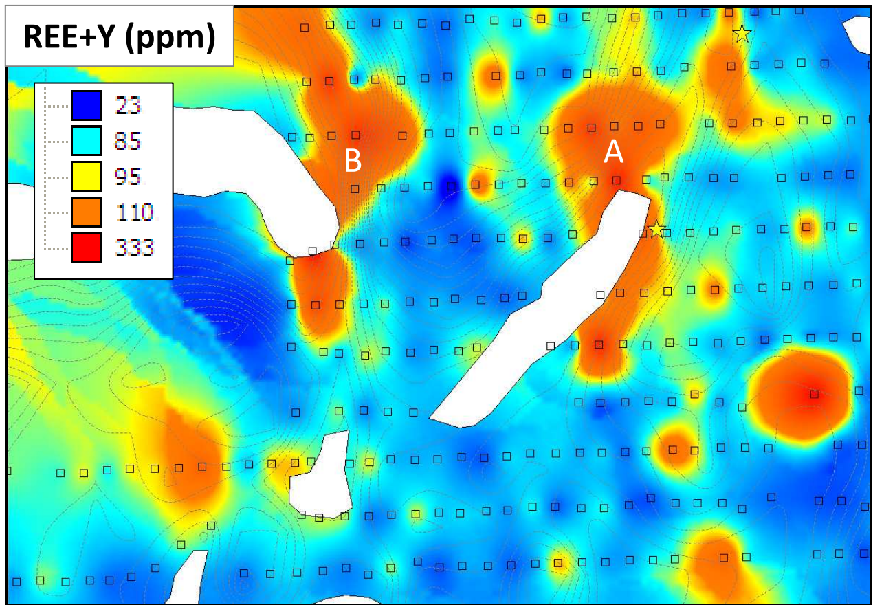
FIGURE 2. SOIL ANOMALIES, B HORIZON, SURPRISE SHOWING AREA (Squares=collection points at 100m spacing, Stars=showings, Lines=5m contour lines)
