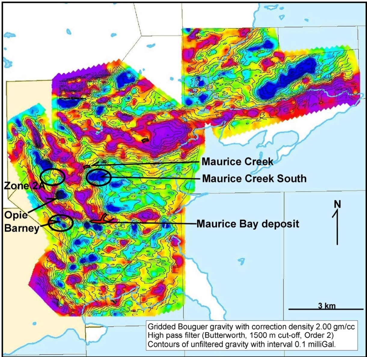
Figure 1: Northwest Athabasca Project Gravity Survey. The proposed 2012 fall drill targets on gravity lows (outlined in blue) are circled in black.
