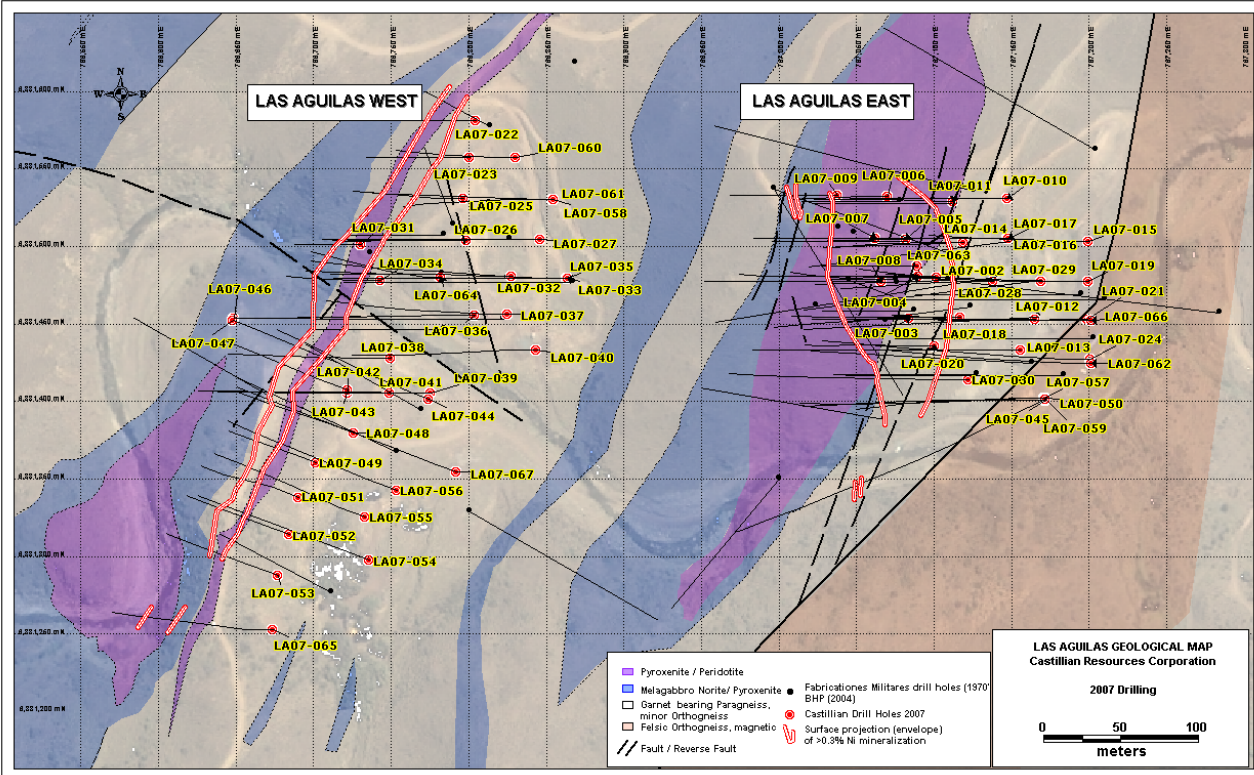
Figure 2: Geological Map showing deposits and diamond drilling on the Las Aguilas Deposits, San Luis Province, Argentina.
