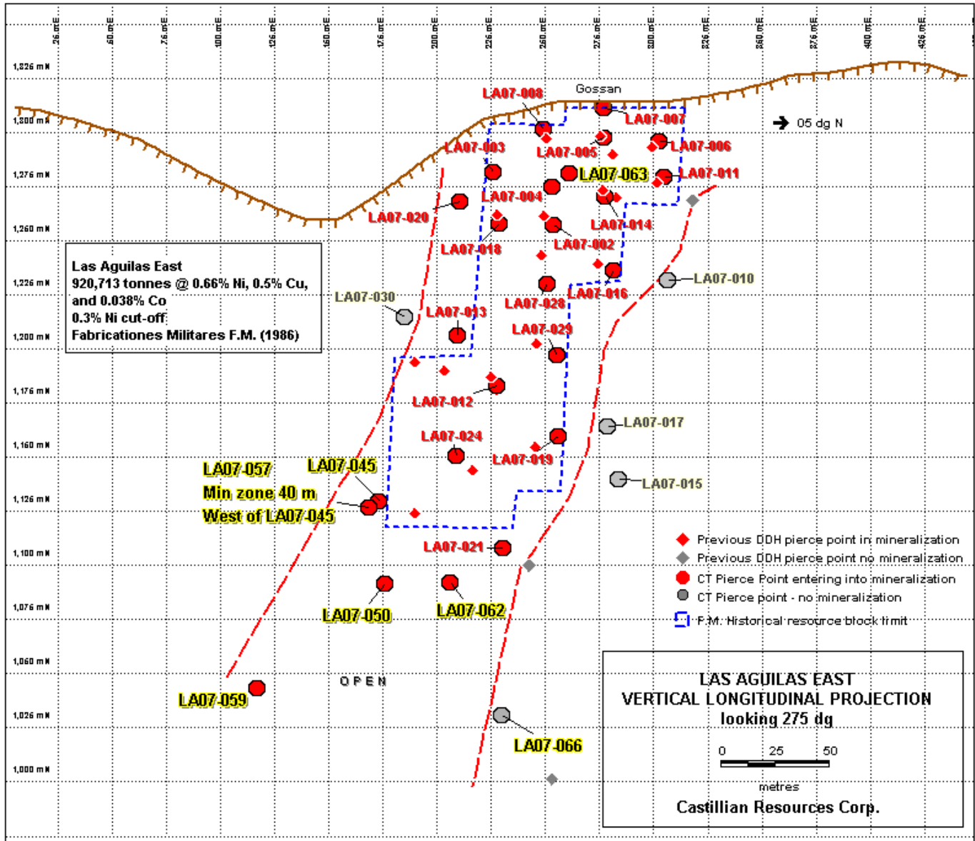
Figure 3: Vertical longitudinal section showing drill hole intercepts for the Las Aguilas East Deposit, San Luis Province, Argentina.
