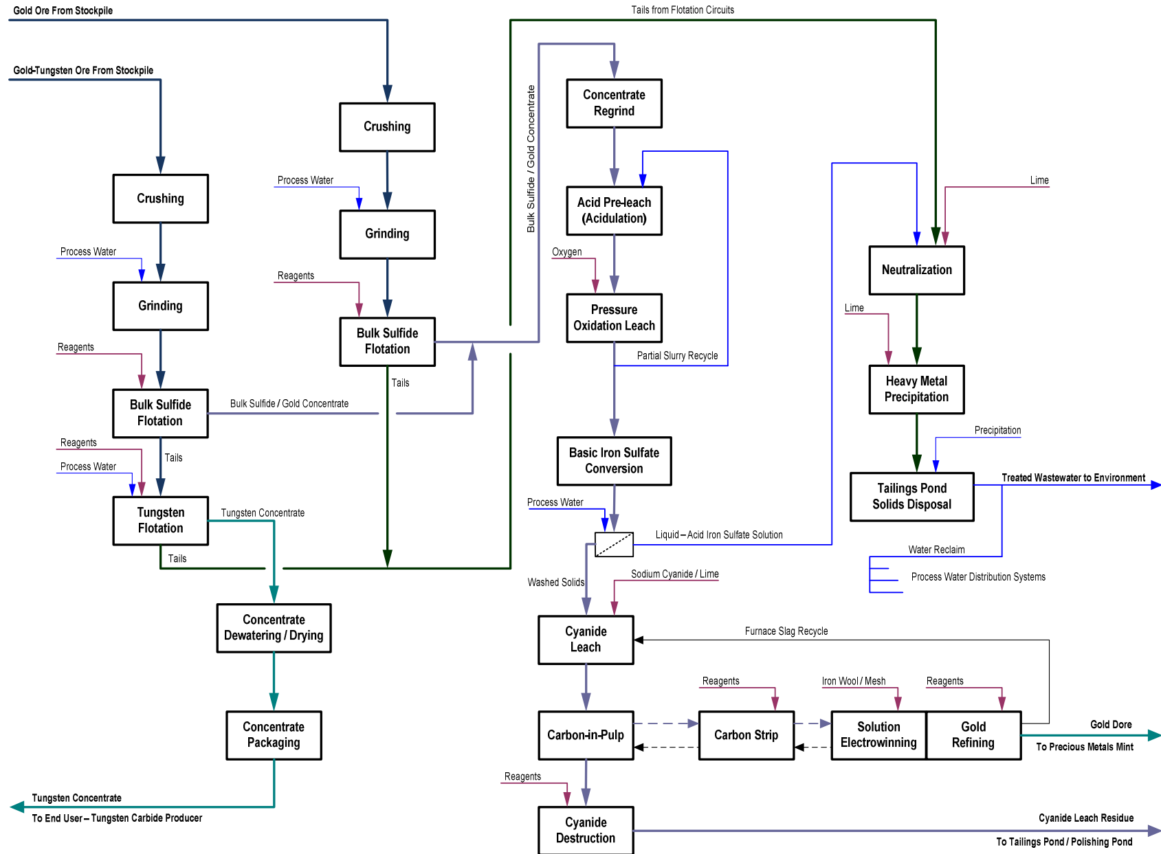
Figure 1: Block Diagram of the Twin Lakes Process Technology
