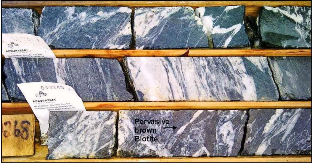
Figure 1: Strongly altered and sheared zone in Balmer basalt at 2268 m, MH1103.
