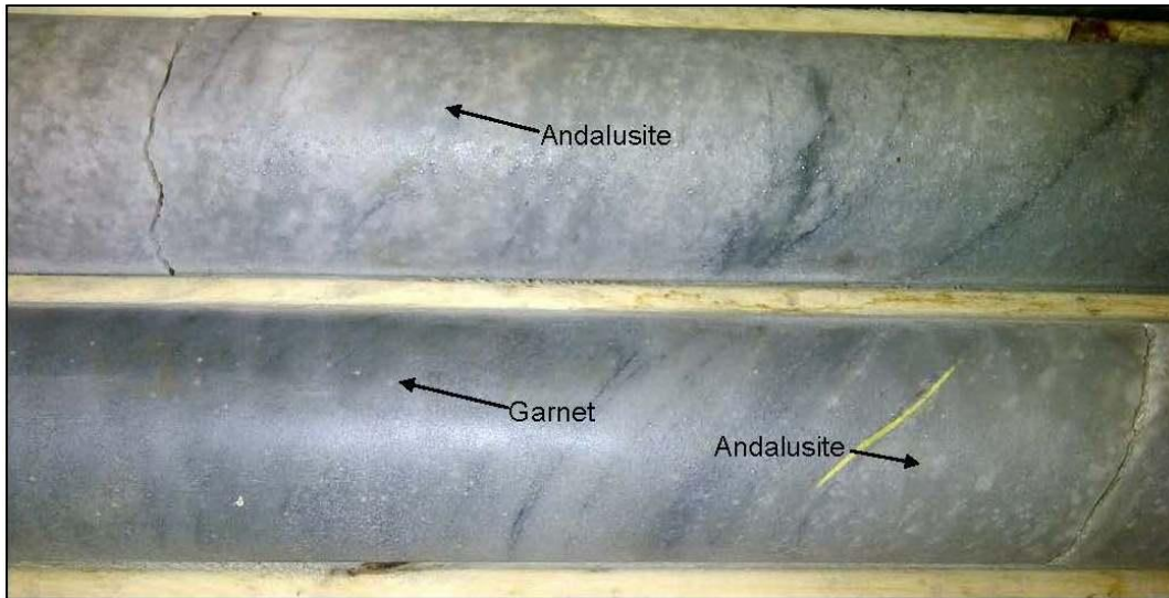
Figure 2: “Bleached basalt”, strongly-altered Balmer Assemblage Basalt or “Campbell-Dickenson Diorite” around 2644 m, MH1103
