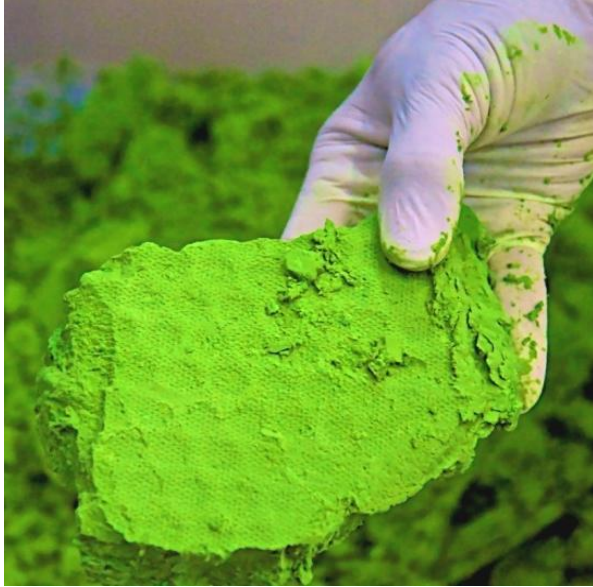
The first NHP 'cake' was produced during the Agata Pilot Plant test at Intertek Minerals Philippines and achieved the expected 52% to 54% nickel grade
