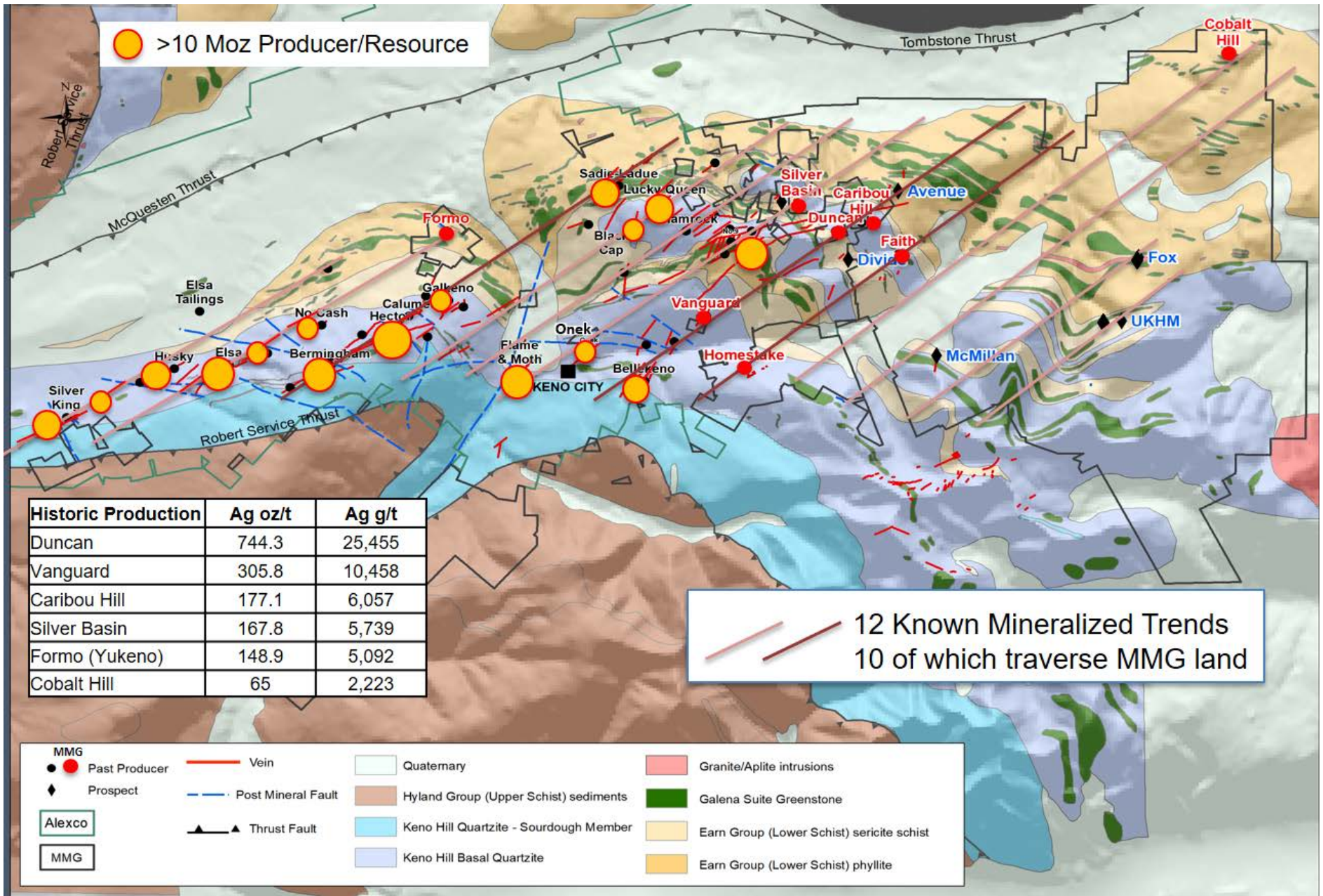
Figure 2: Keno District Geology and Structural Trends
